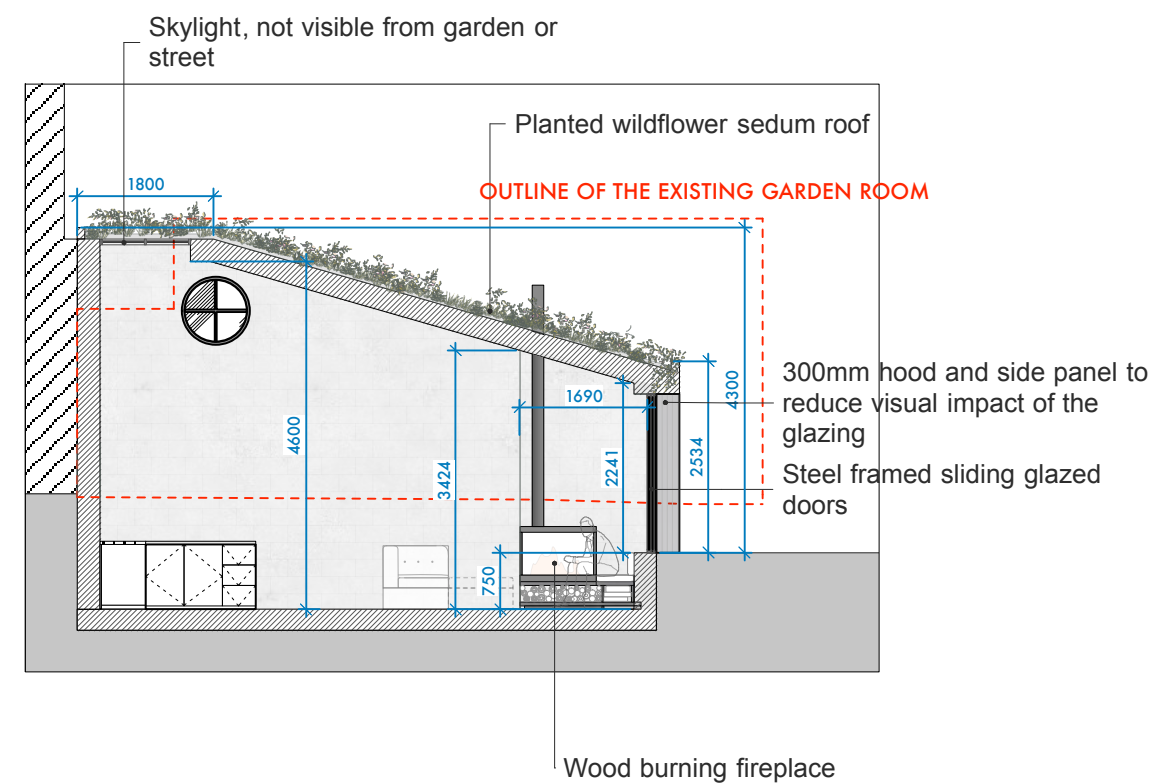
Section BB
