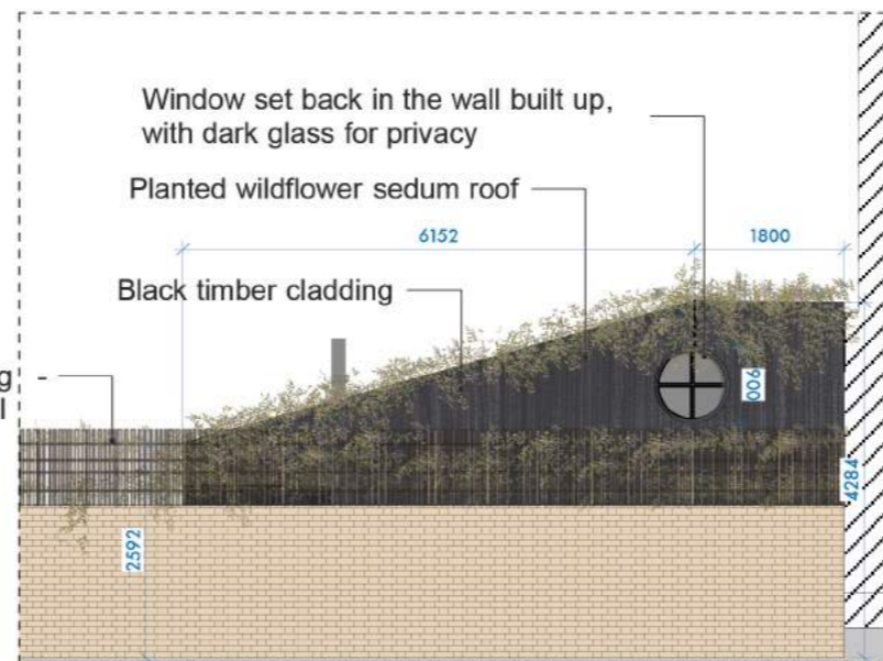
North-East Elevation
