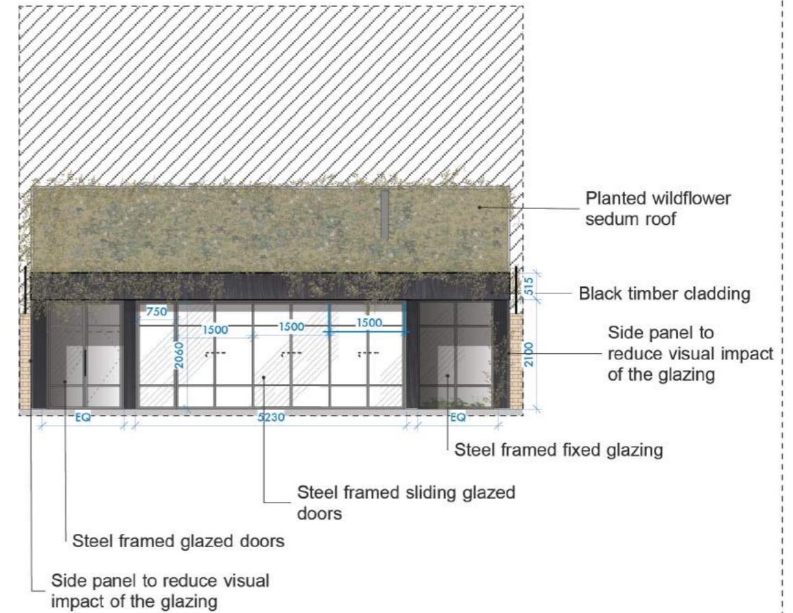
Front Elevation
