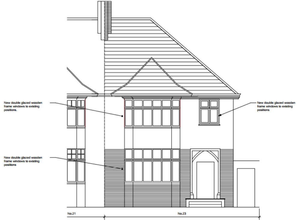
2 Proposed Front Elevation Scale: 1:50
