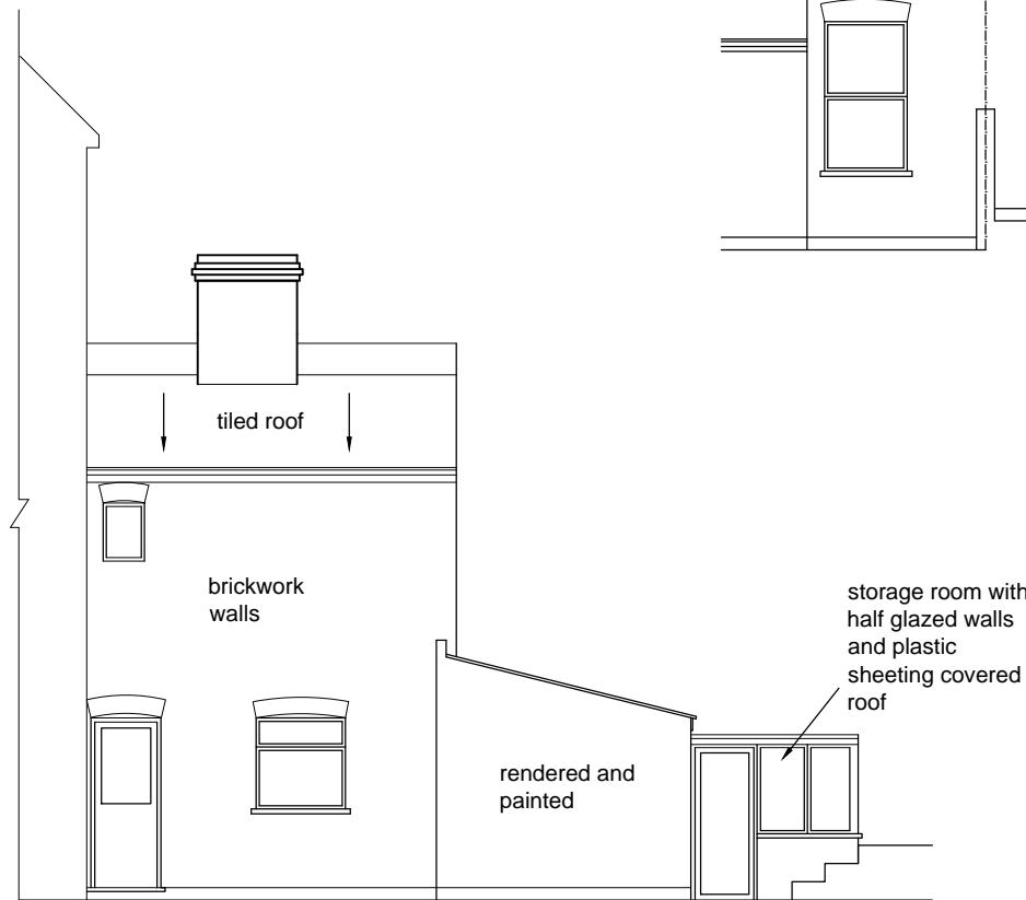
Back Addition Side Elevation 'As Existing' S: 1/100
