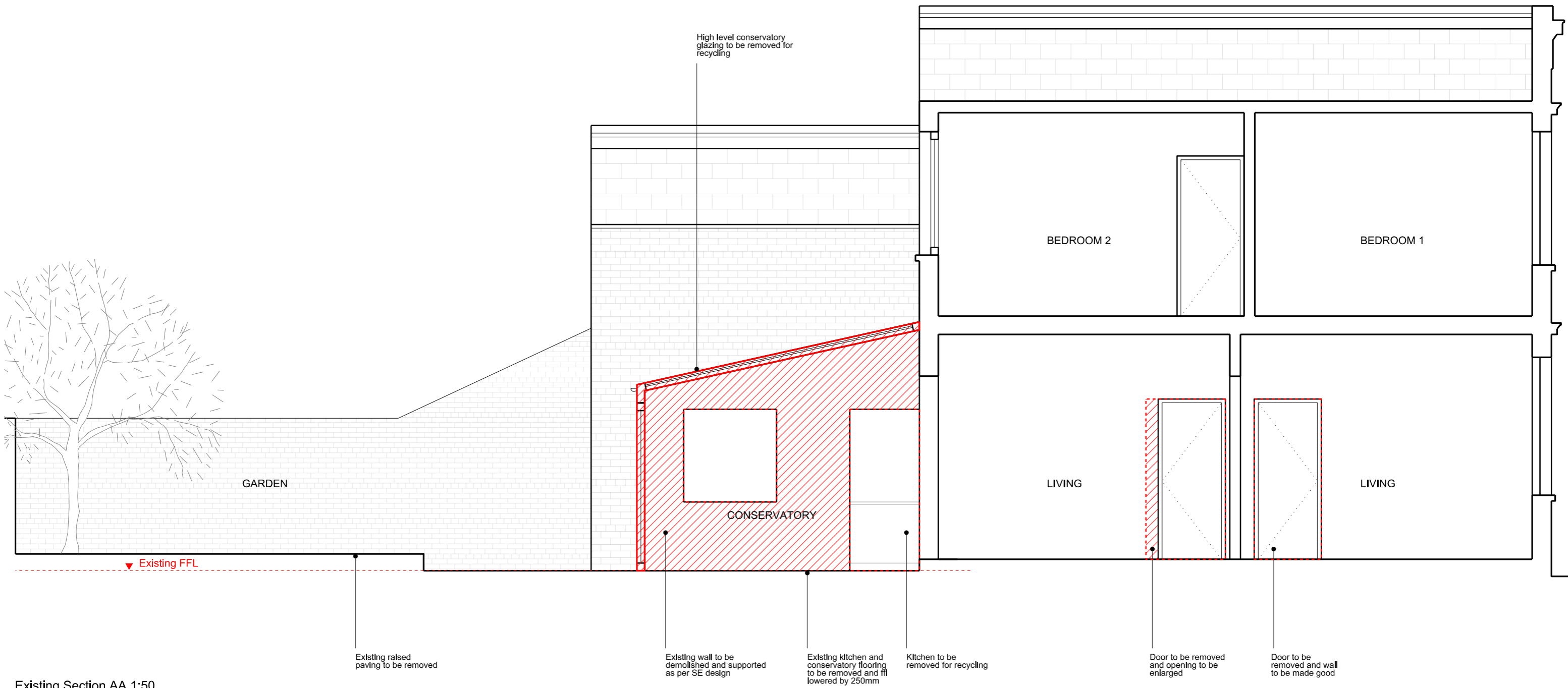
Existing Section AA 1:50
