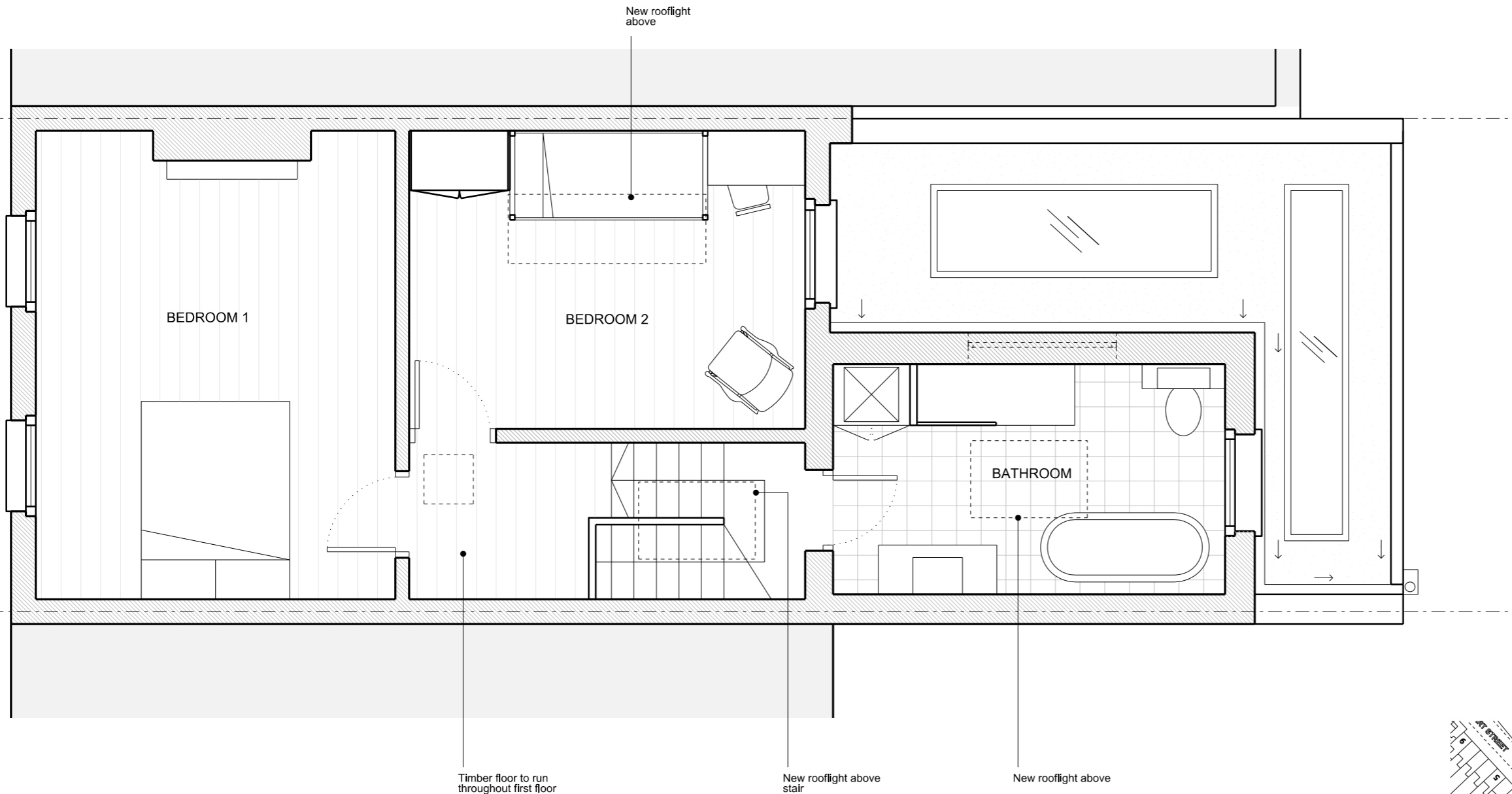
PROPOSED FIRST FLOOR PLAN 1:50
