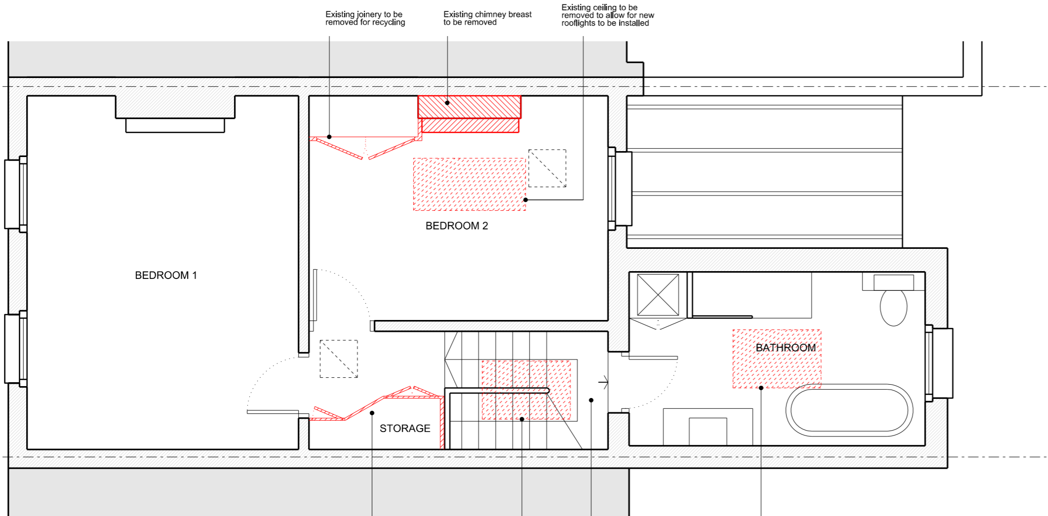
EXISTING FIRST FLOOR PLAN 1:50
