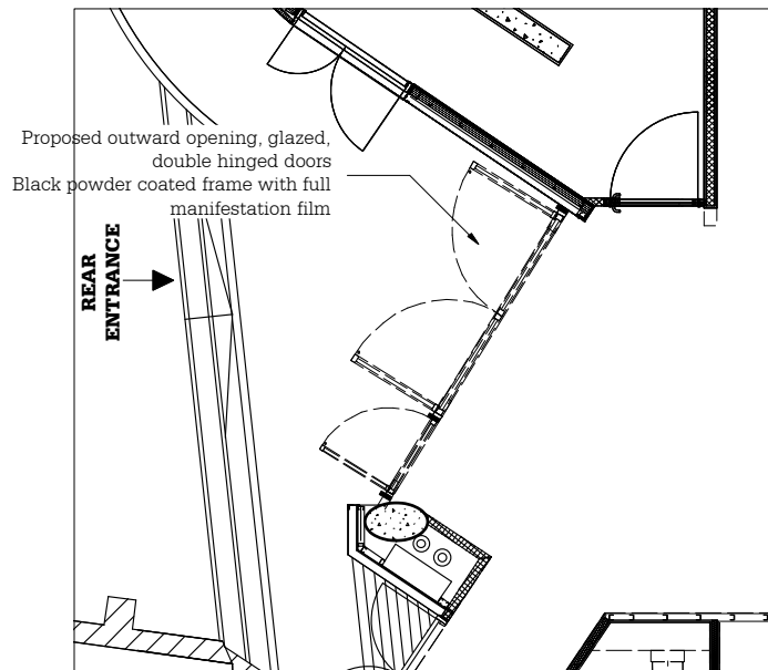
4 Proposed Rear (West) Entrance Door PL.00 1:100 @ A3
