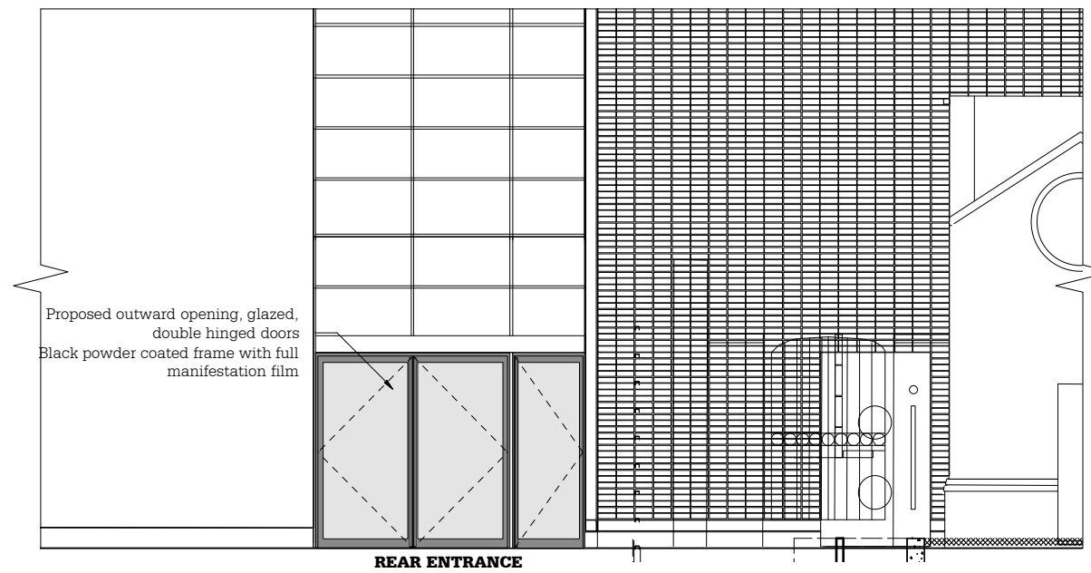
5 Proposed Rear (West) Elevation PL.00 1:100 @ A3
