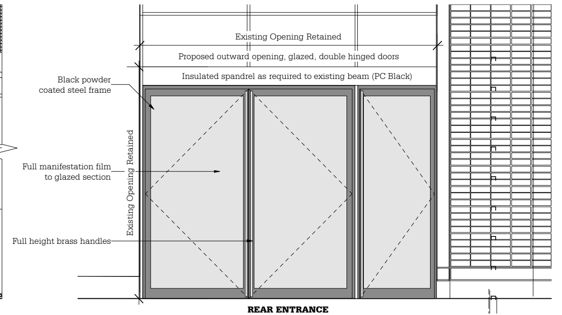
6 Proposed Rear (West) Elevation PL.00 1:50 @ A3
