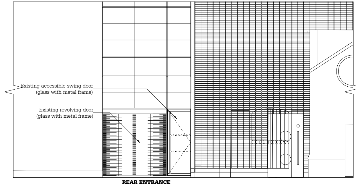
2 Existing Rear (West) Elevation PL.00 1:100 @ A3
