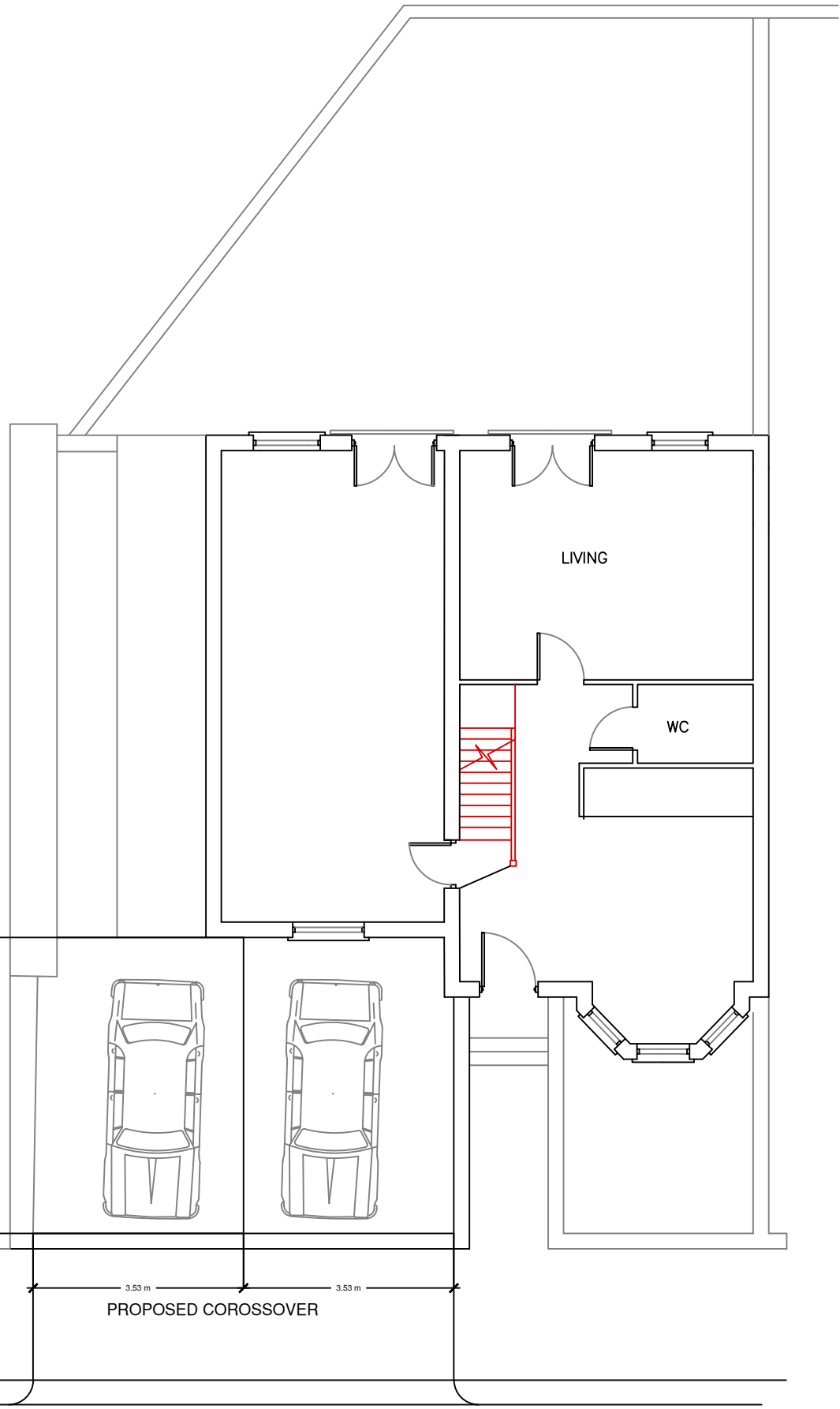
GROUND FLOOR PLAN SHOWING NEW FRONT CAR PARKING SPACES
