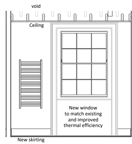
Elevation D
