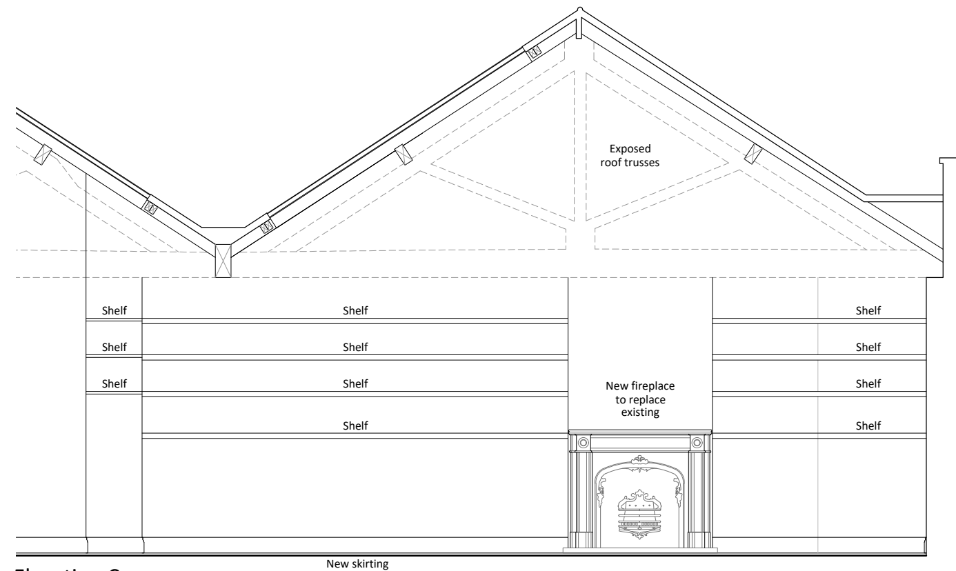
Elevation C
