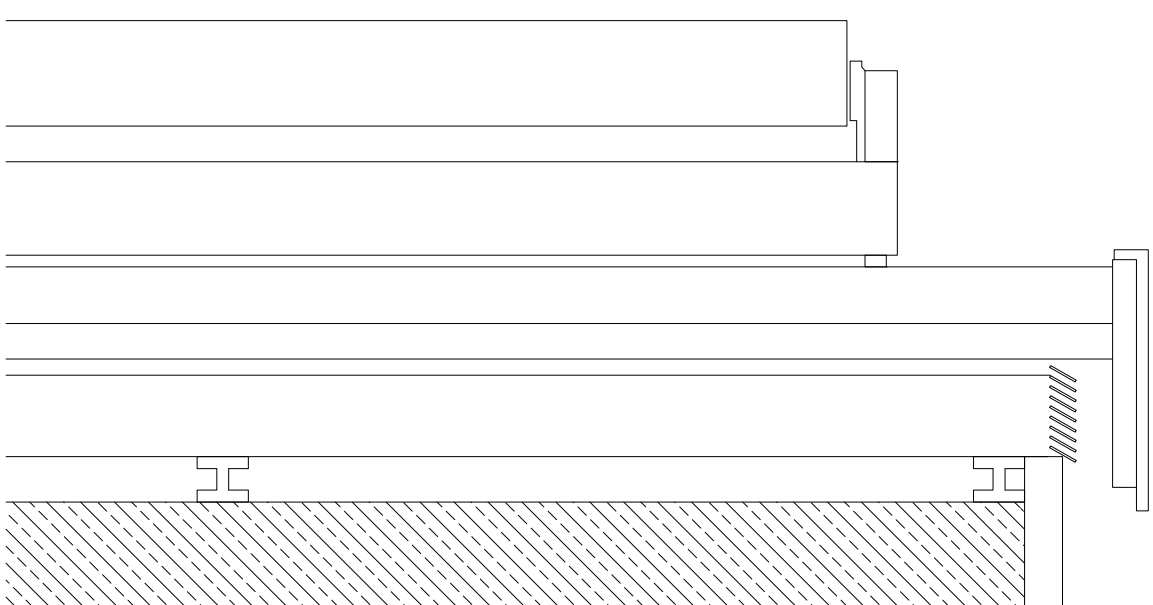
04 Section A-A' Scale 1.20
