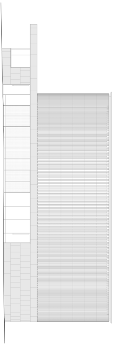
01 Existing elevation east
