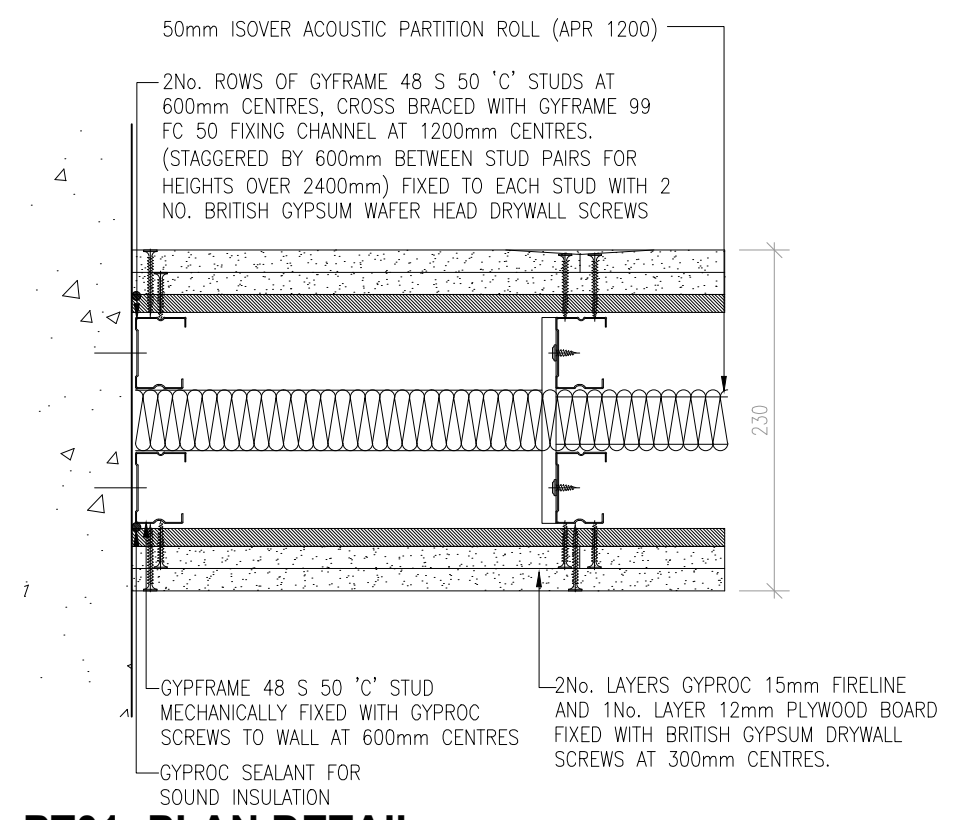
PT01: PLAN DETAIL SCALE: 1:5
