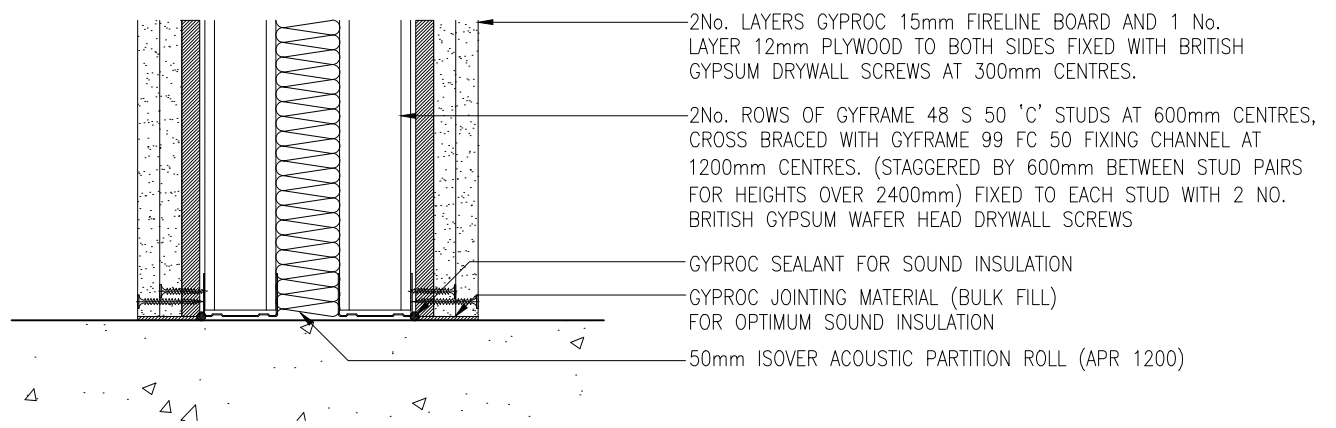
PT01: BASE DETAIL SCALE: 1:5
