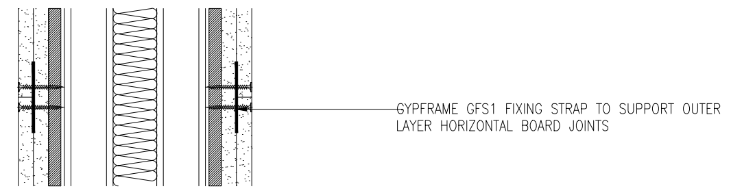
PT01: HEAD DETAIL SCALE: 1:5
