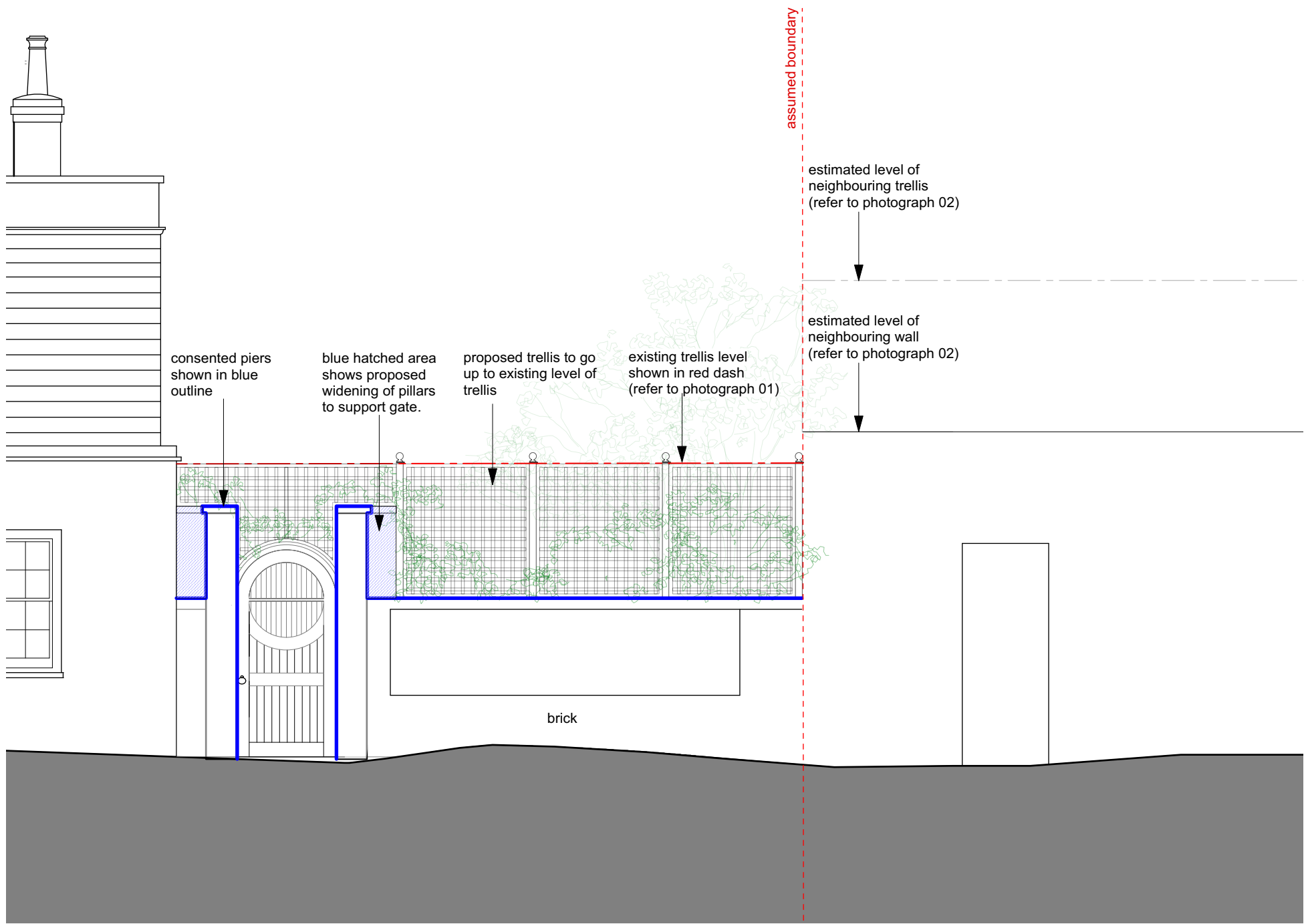
Proposed rear garden wall and gate (explanatory sketch)
