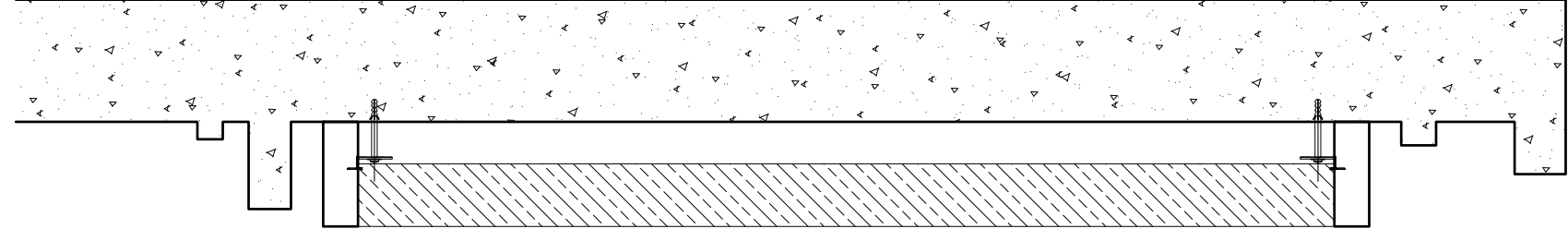
04 Section A-A' Scale 1.20
