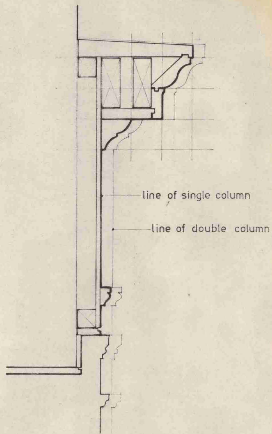
SECTION THRO' FASCIA 1:5
