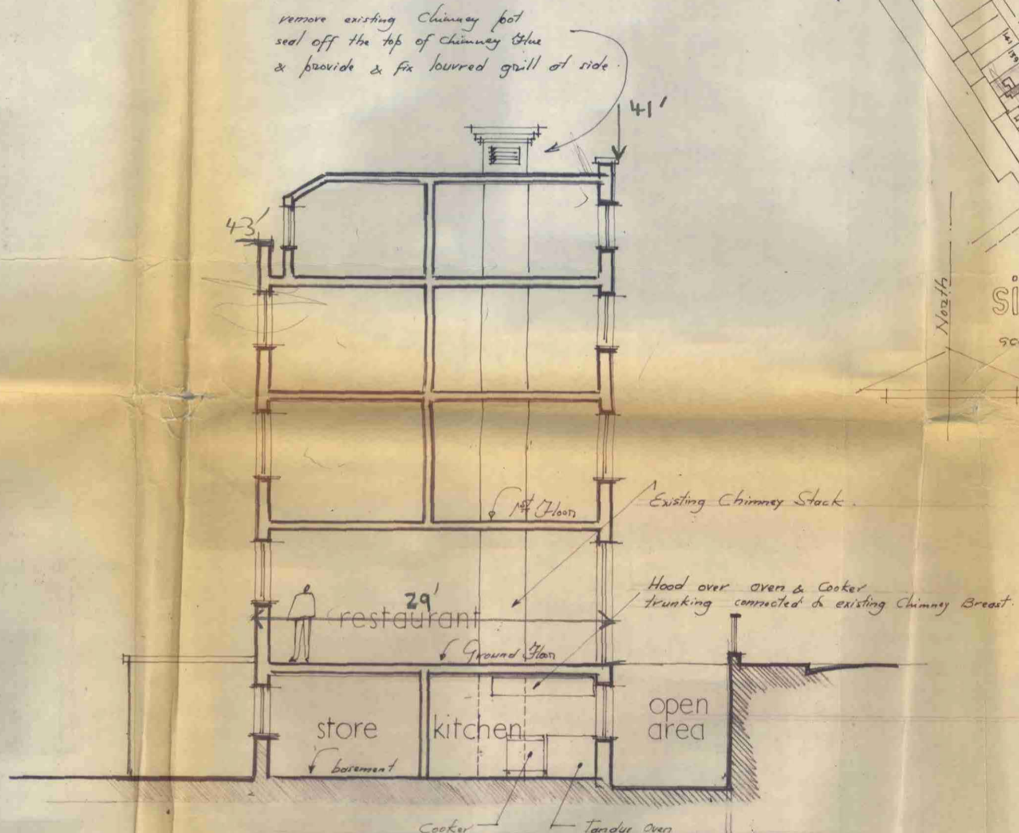
section X X scale: eight feet to an inch.
