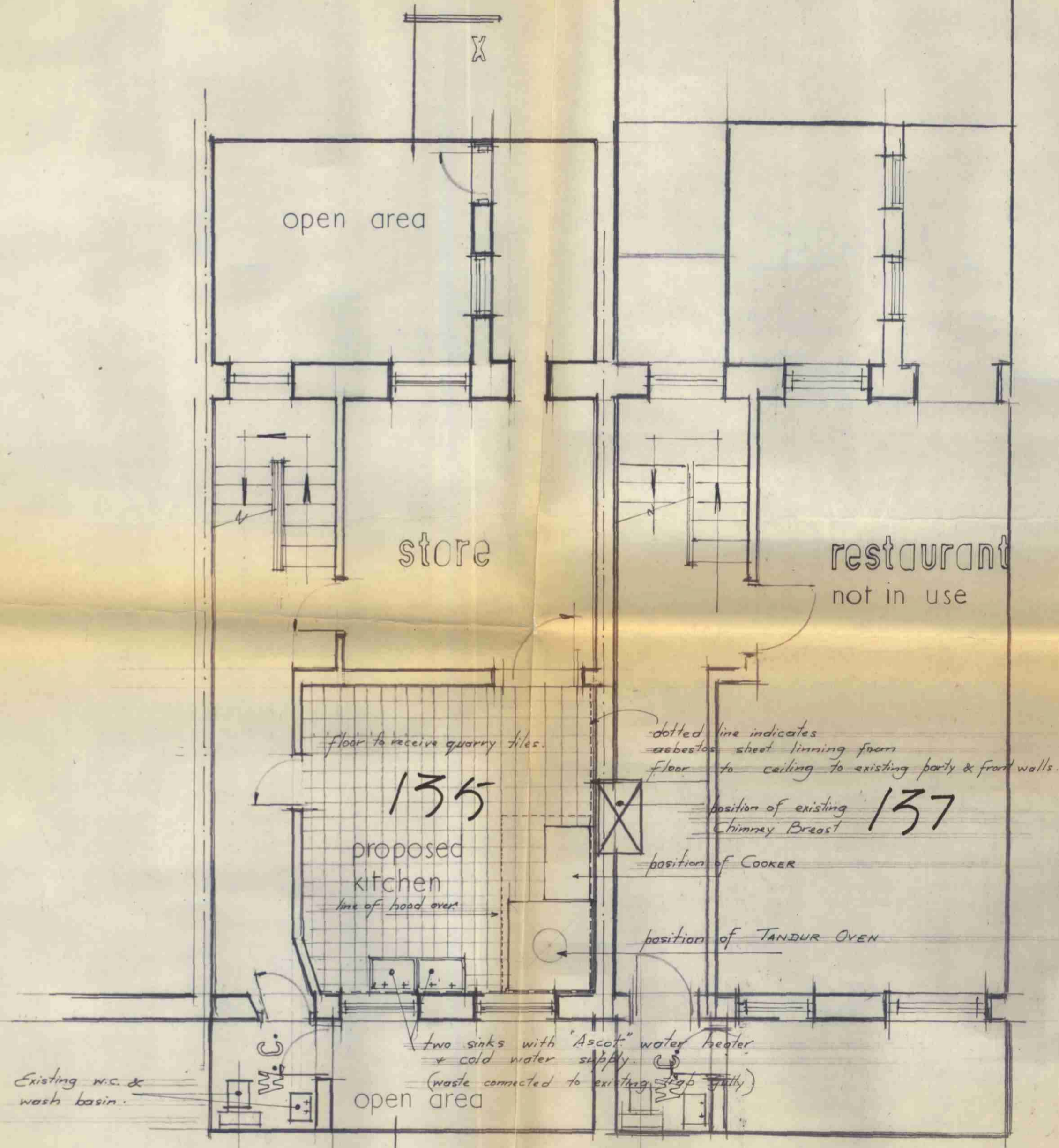
basement scale: four feet to an inch.
