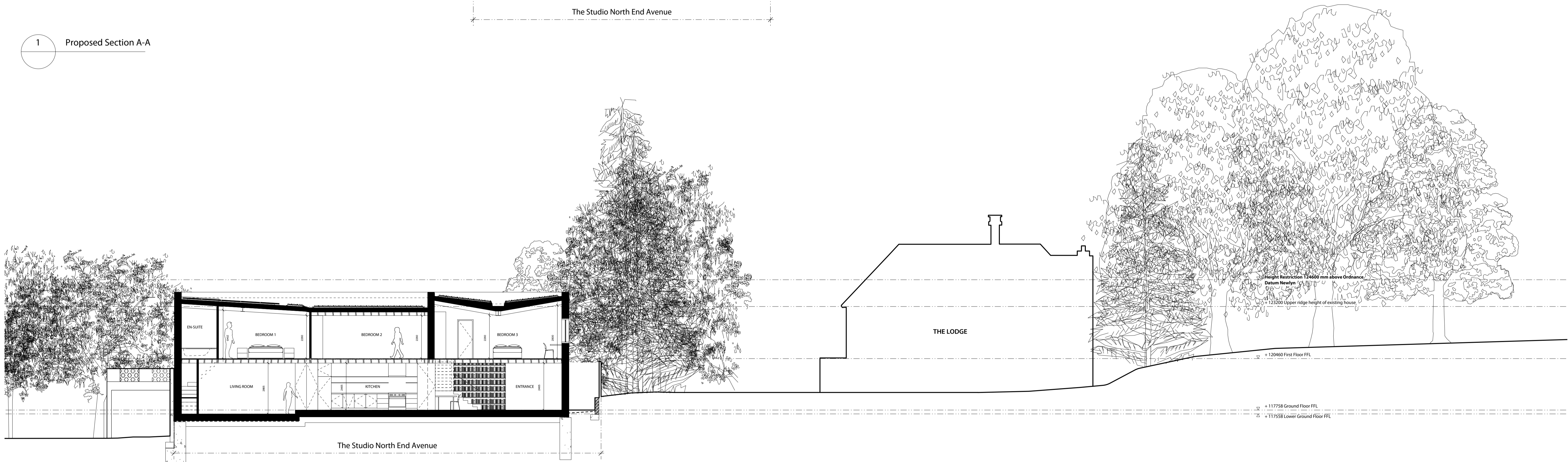
2 Proposed Section D-D
