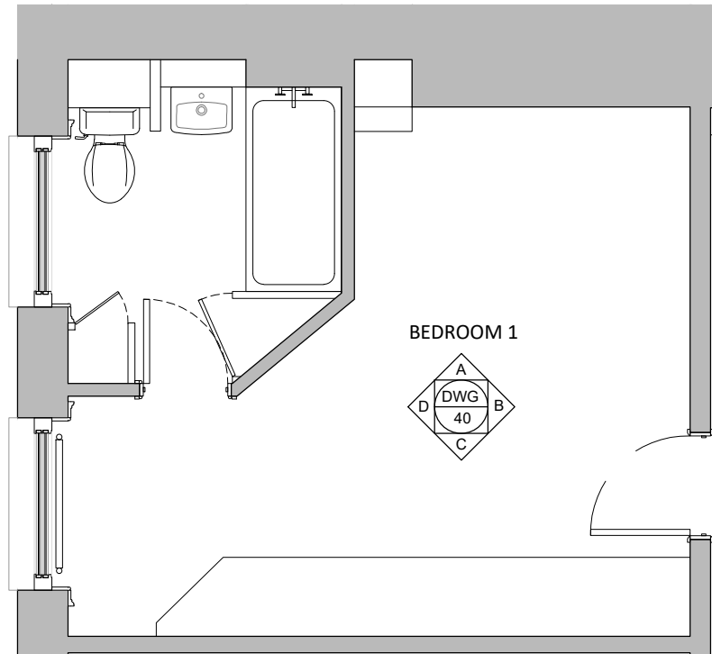
Room Plan
