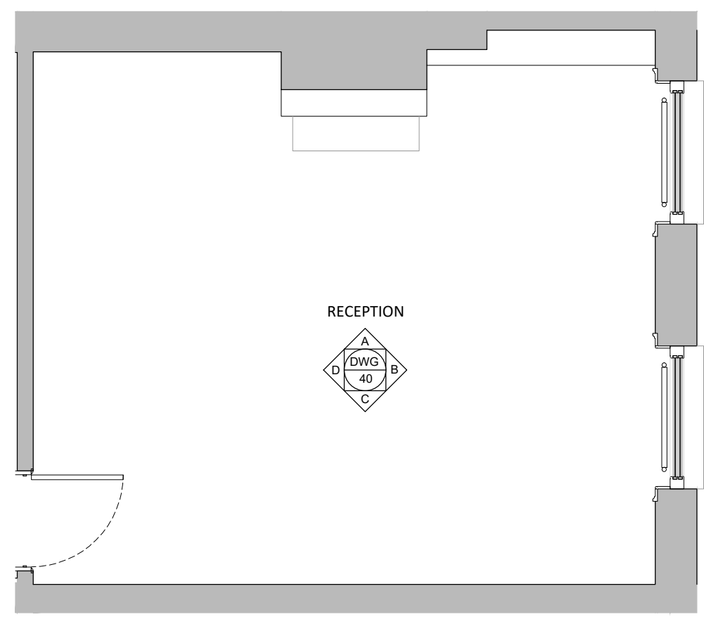
Room Plan
