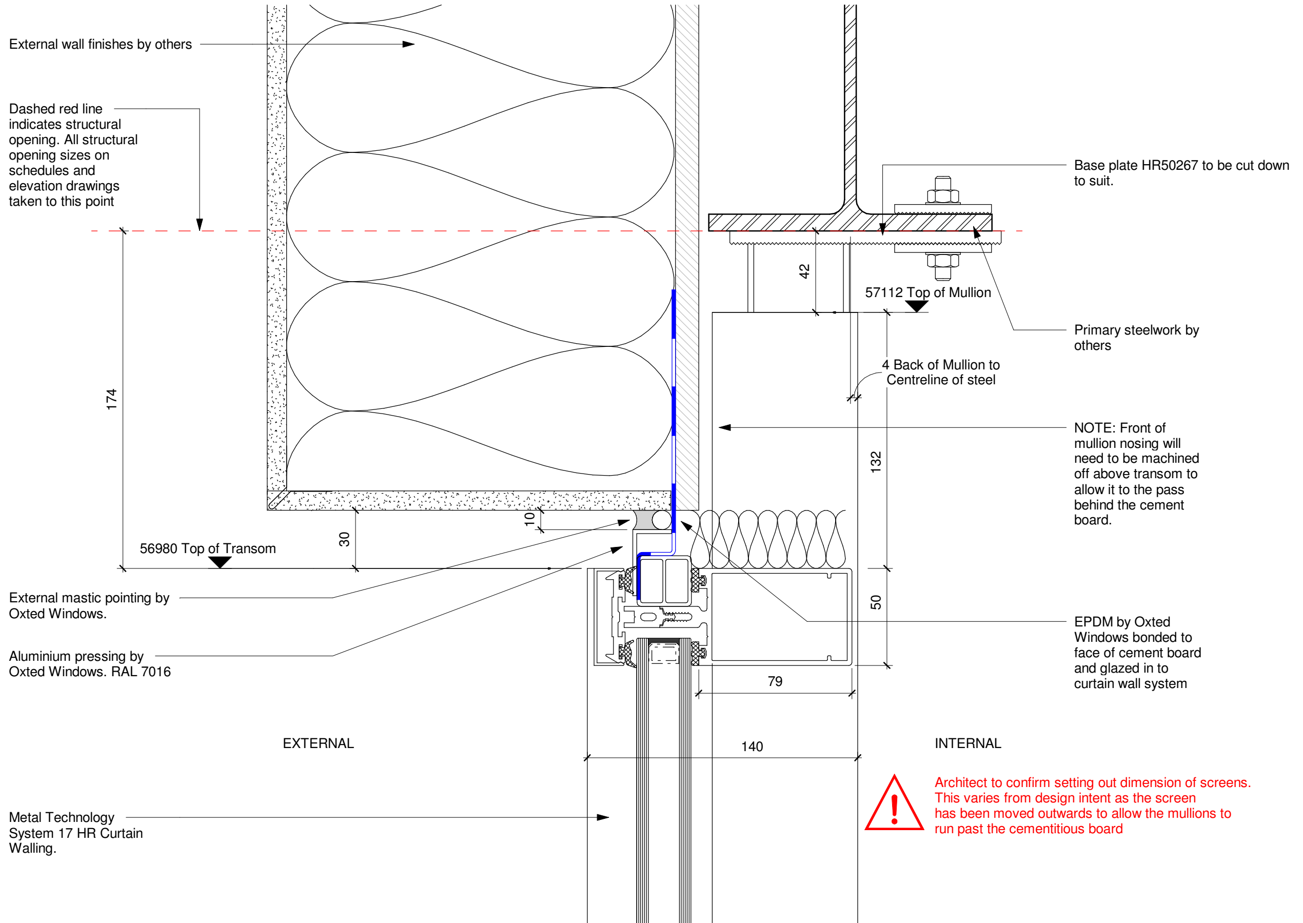
1 Typical Head Detail Type 3 A140 1 : 2
