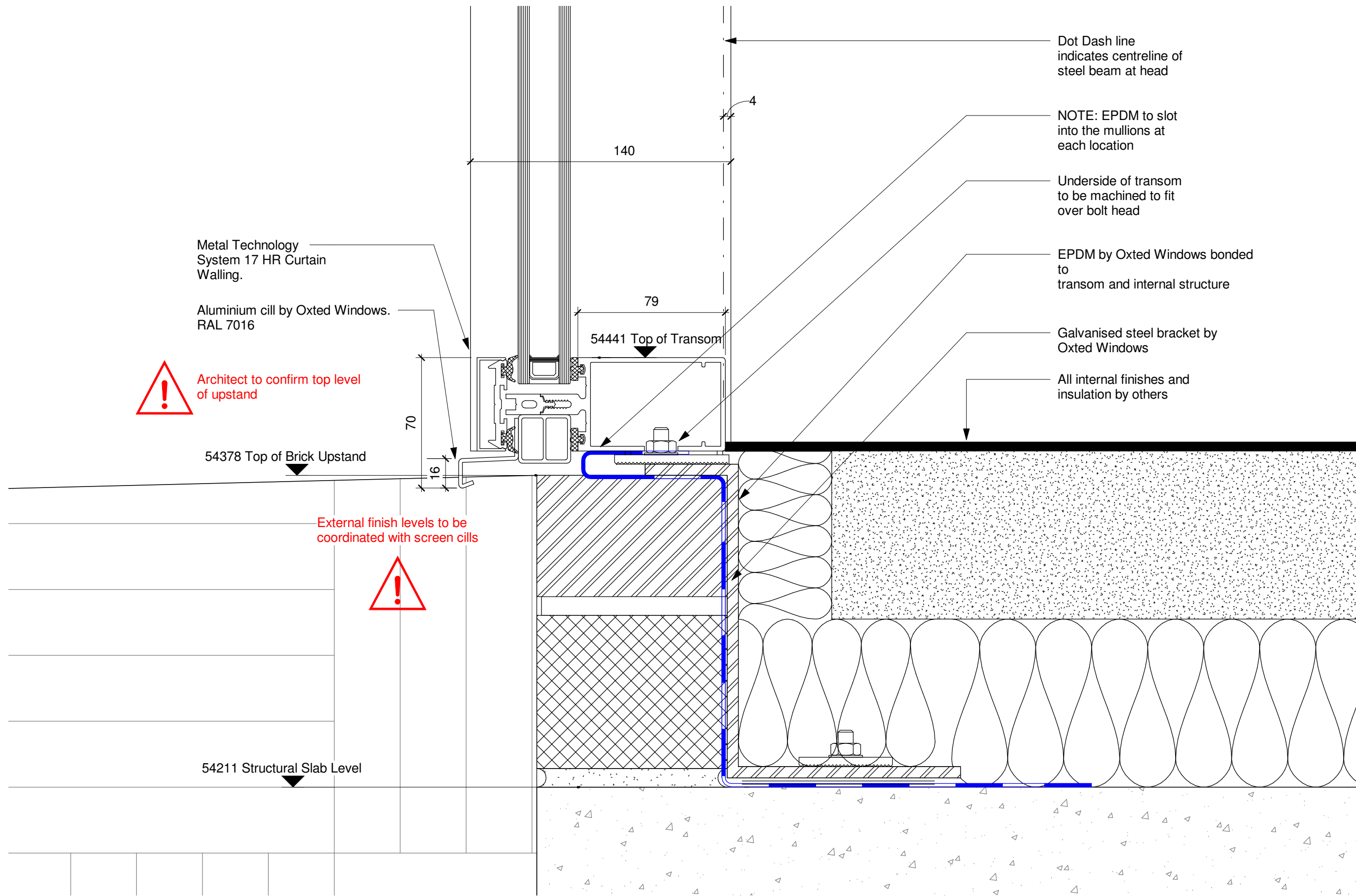
1 Typical Cill Detail Type 5 A136 1 : 2
