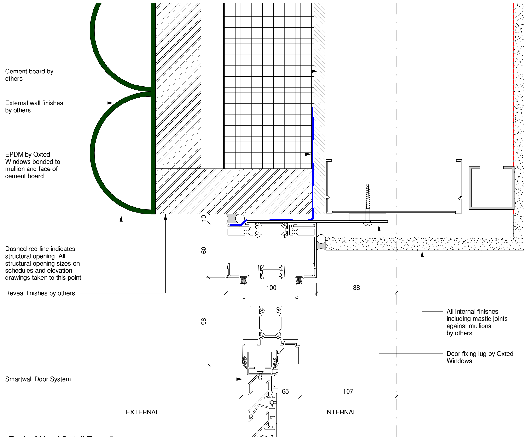
1 Typical Head Detail Type 5 A134 1 : 2
