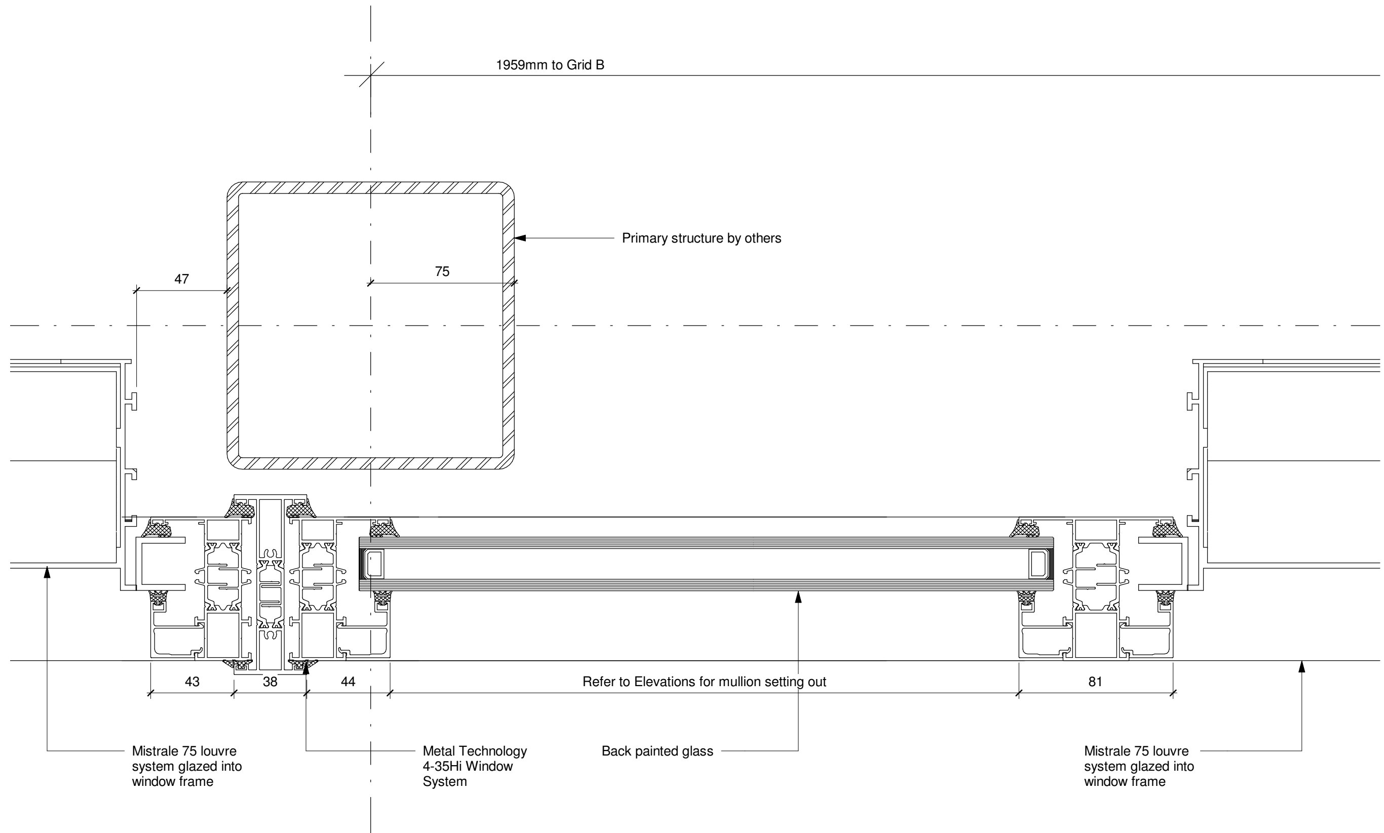
1 Typical Jamb Detail Type 8 A130 1:2
