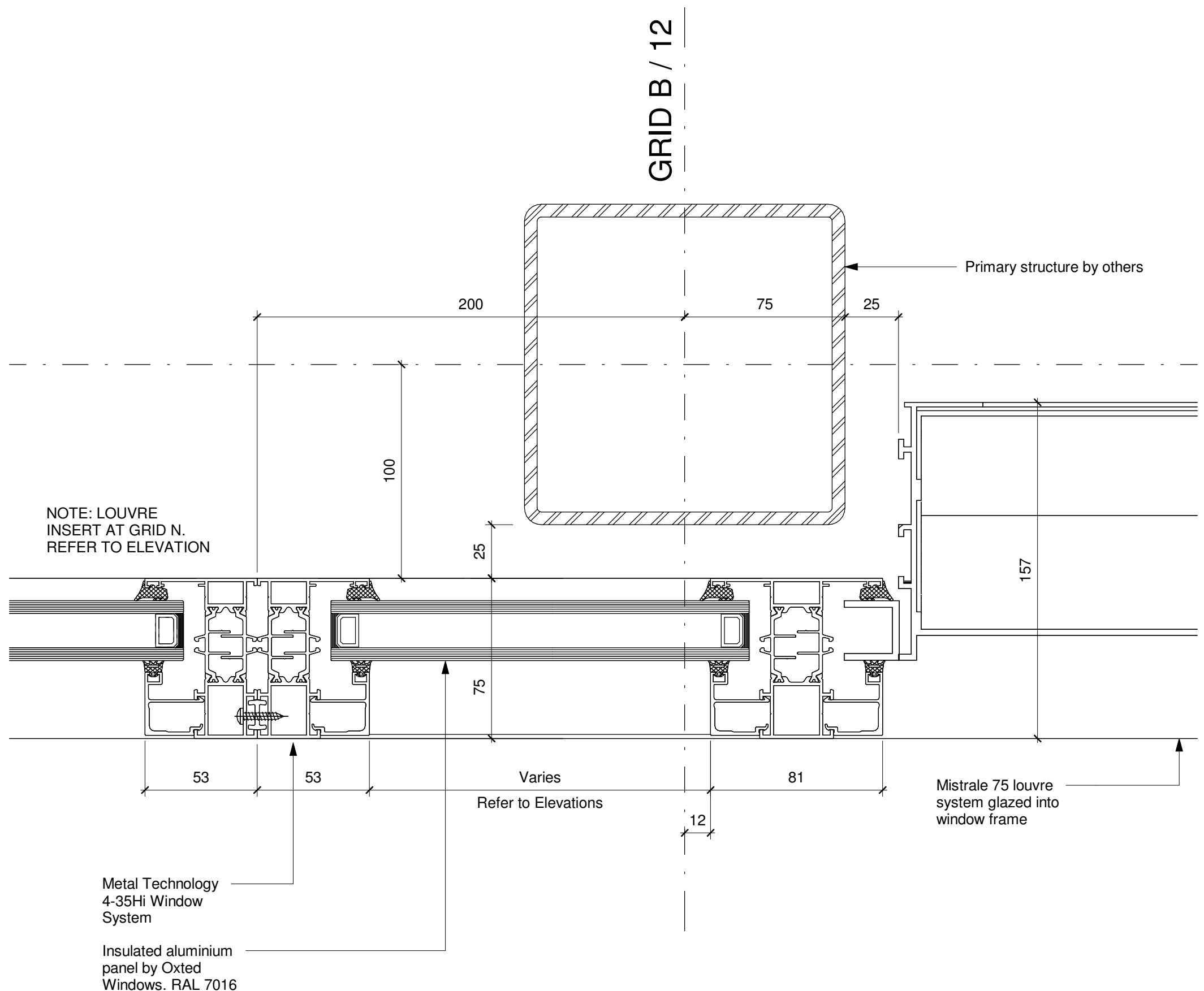
1 Typical Jamb Detail Type 7 A129 1 : 2
