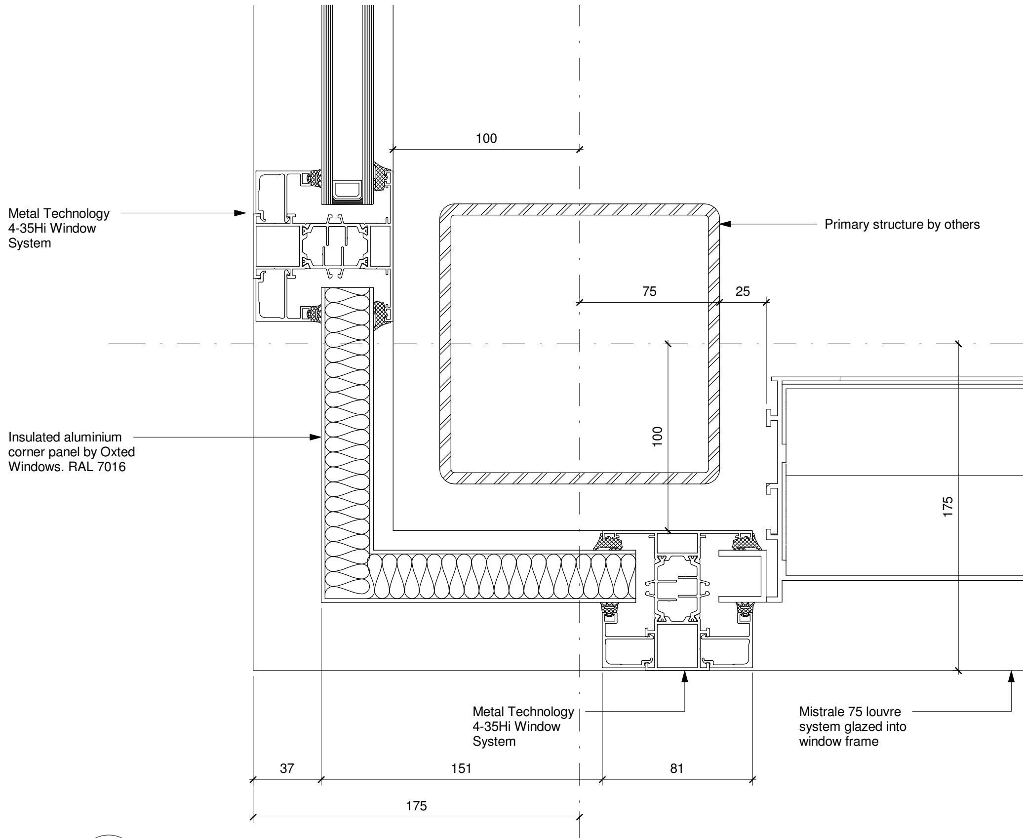
1 Typical Jamb Detail Type 2 A128 1 : 2
