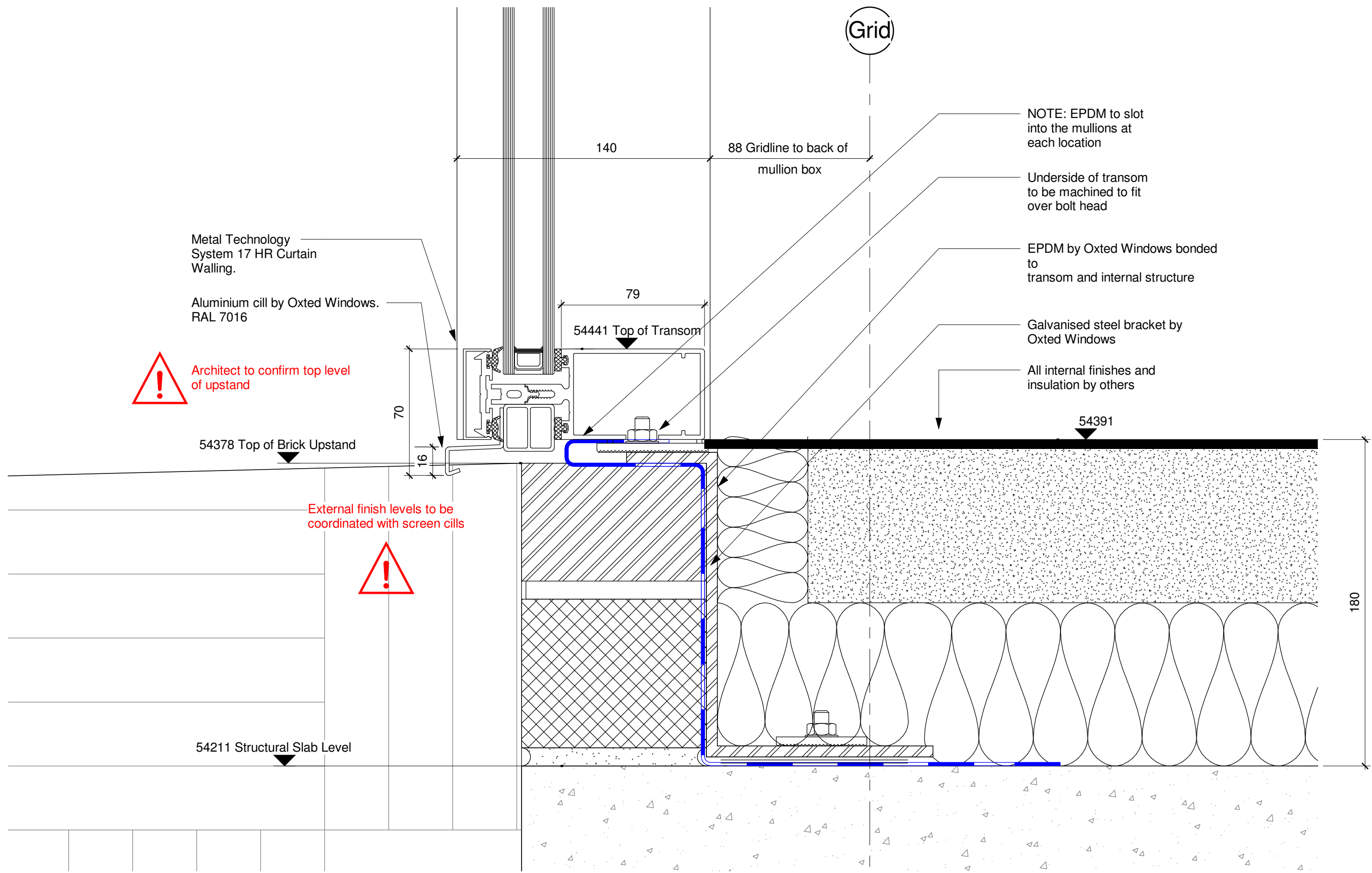
1 Typical Cill Detail Type 1 A122 1 : 2
