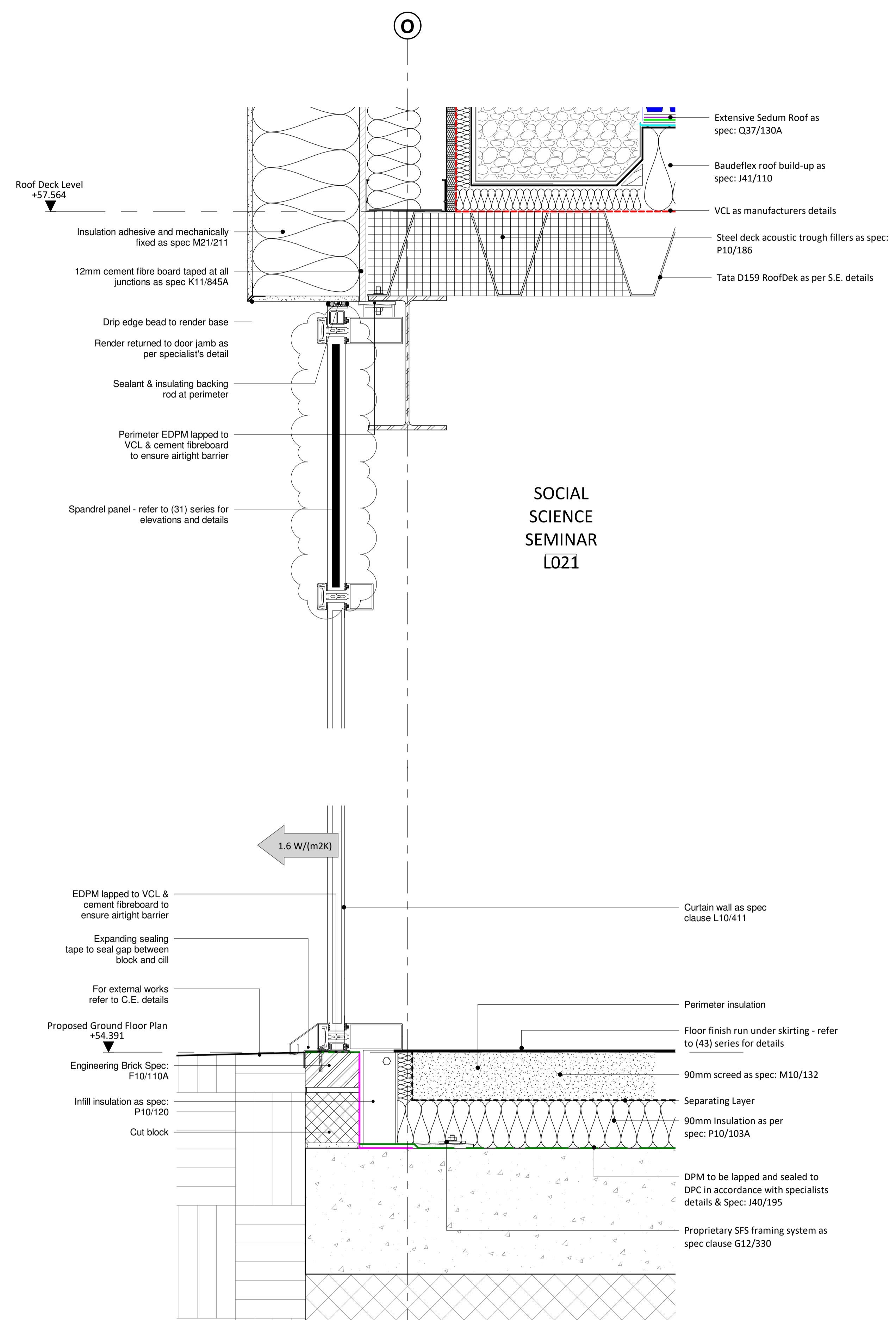
2. Insulated Render & Curtain Wall Head & Cill Section SCALE - 1 : 5@A1
