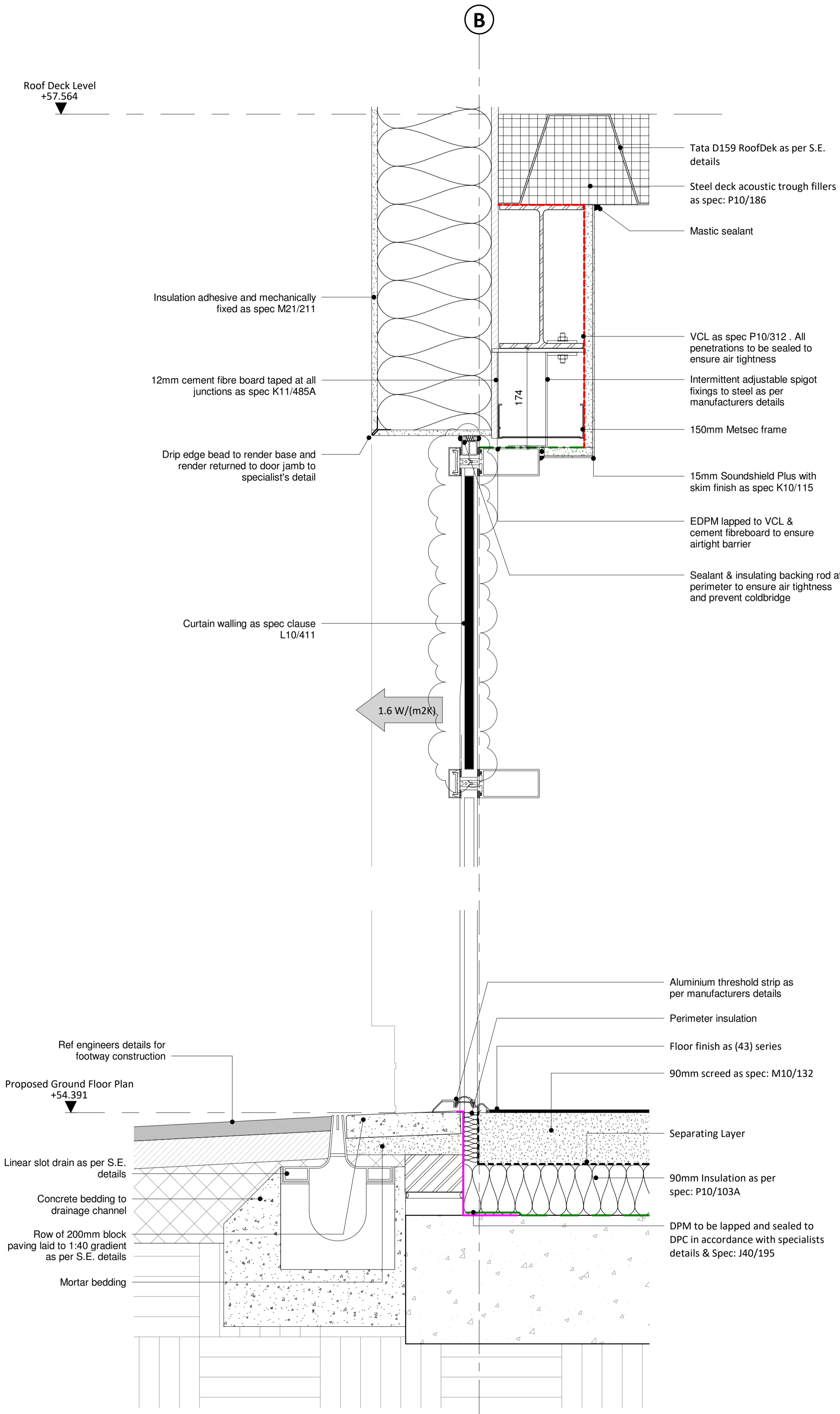
1. Door Head & Threshold Detail SCALE - 1 : 5@A1
