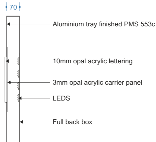
Section Detail A-A 1:10@A3
