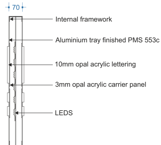
Section Detail B-B 1:10@A3
