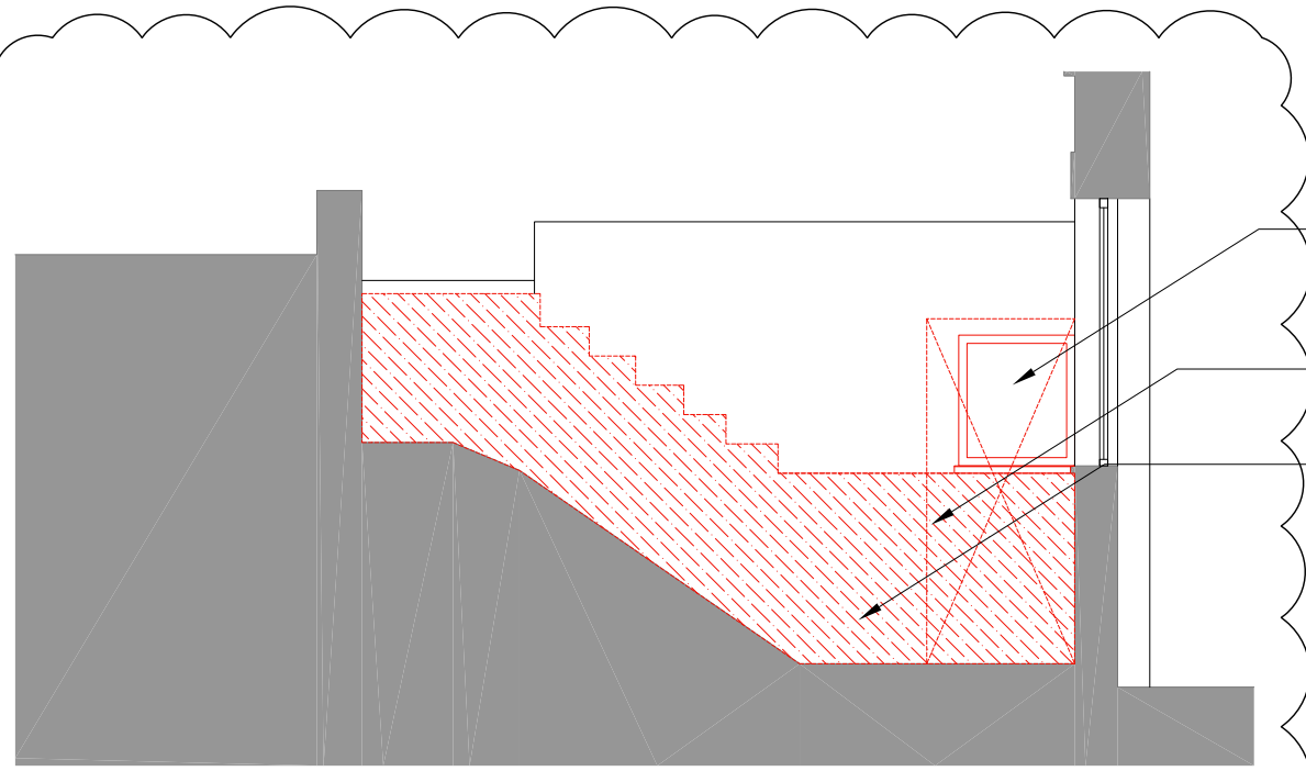
02 SECTION BB Scale: 1:50 SECTION/ELEVATION
