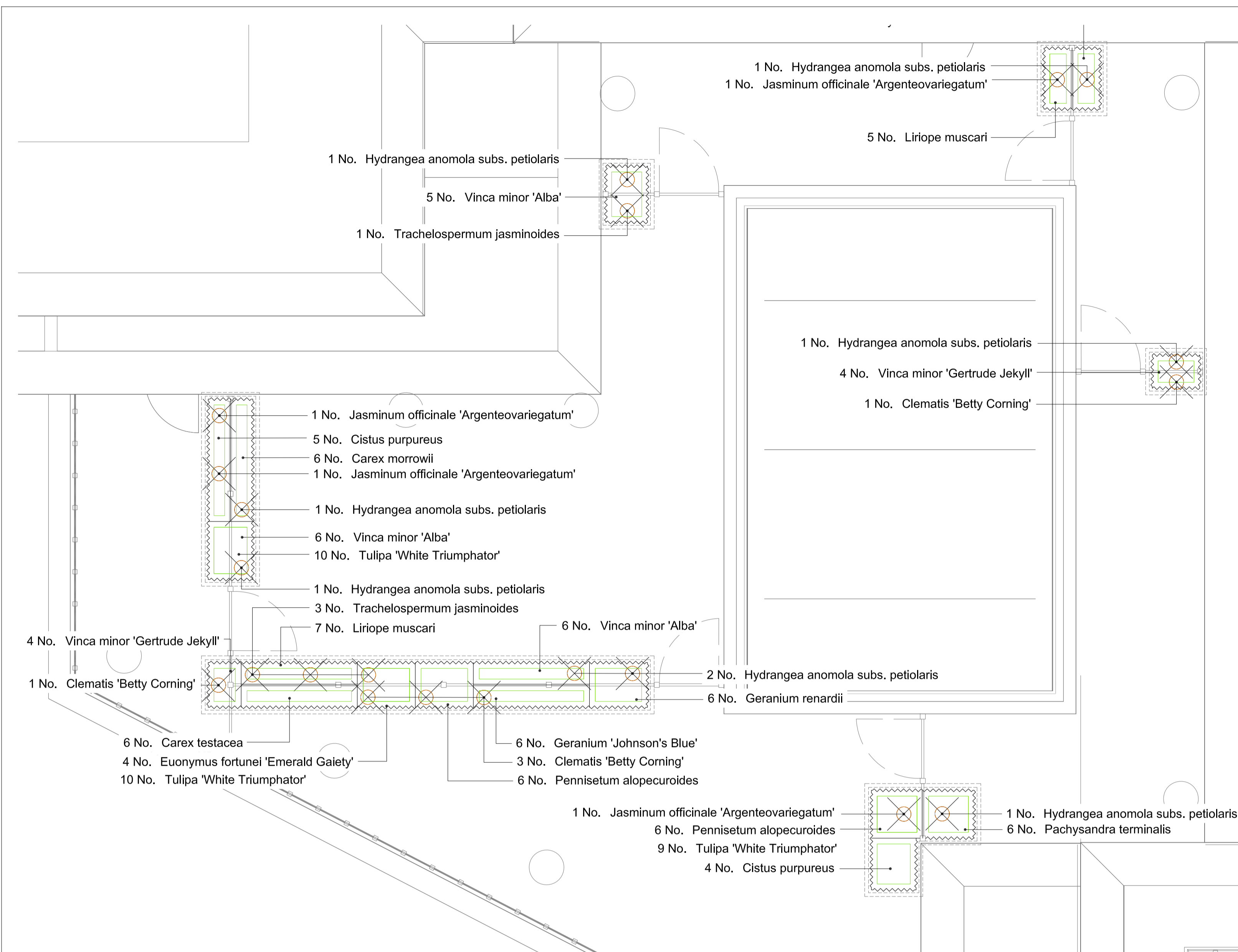
1 Building E: Level 1 Roof Terrace L.323 SCALE 1:50@A1
