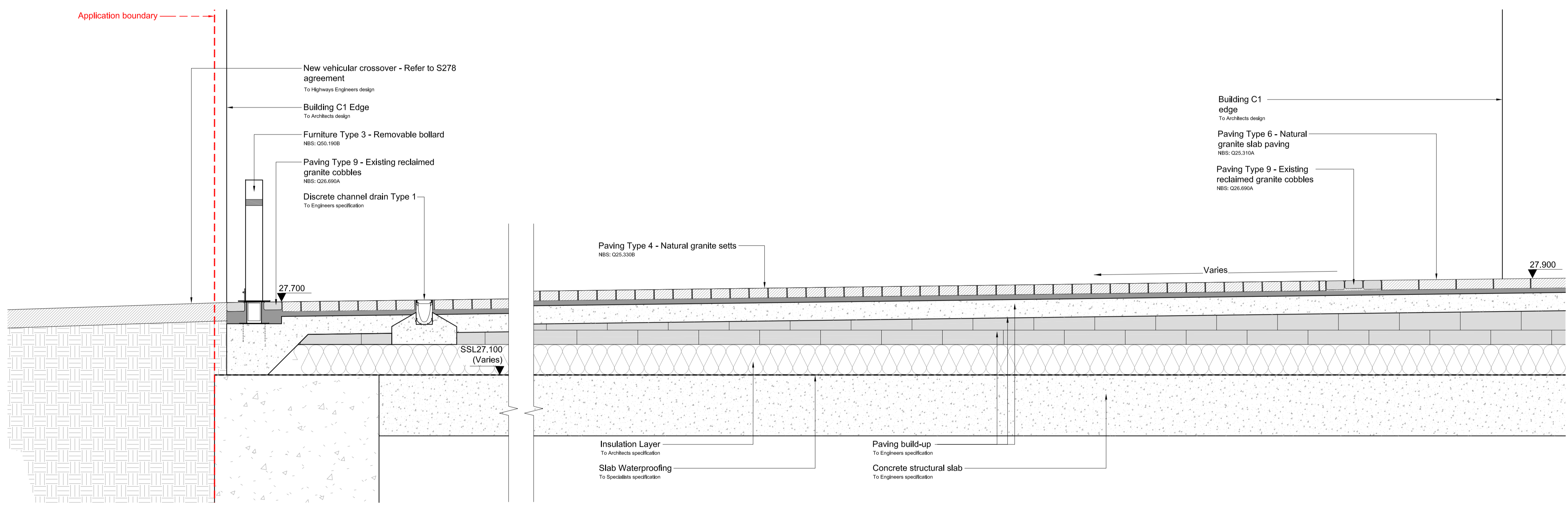
4 Section through local space access from Castlehaven Road SCALE 1:20@A1
