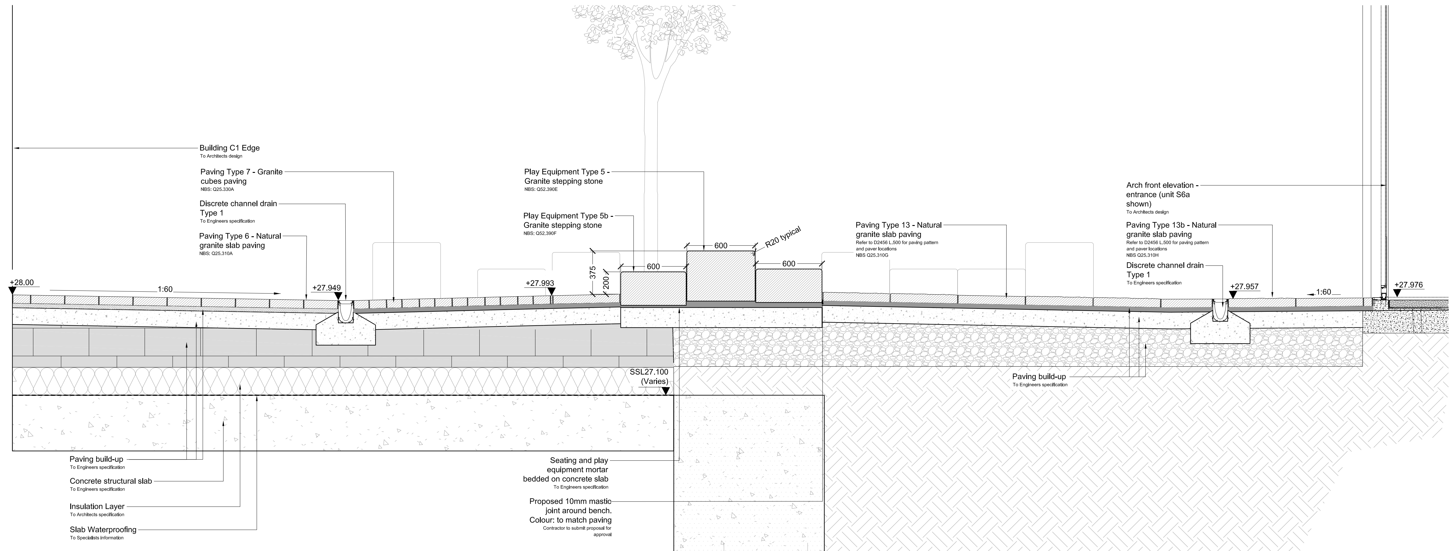
2 Building C1 - Section through local space play area SCALE 1:20@A1
