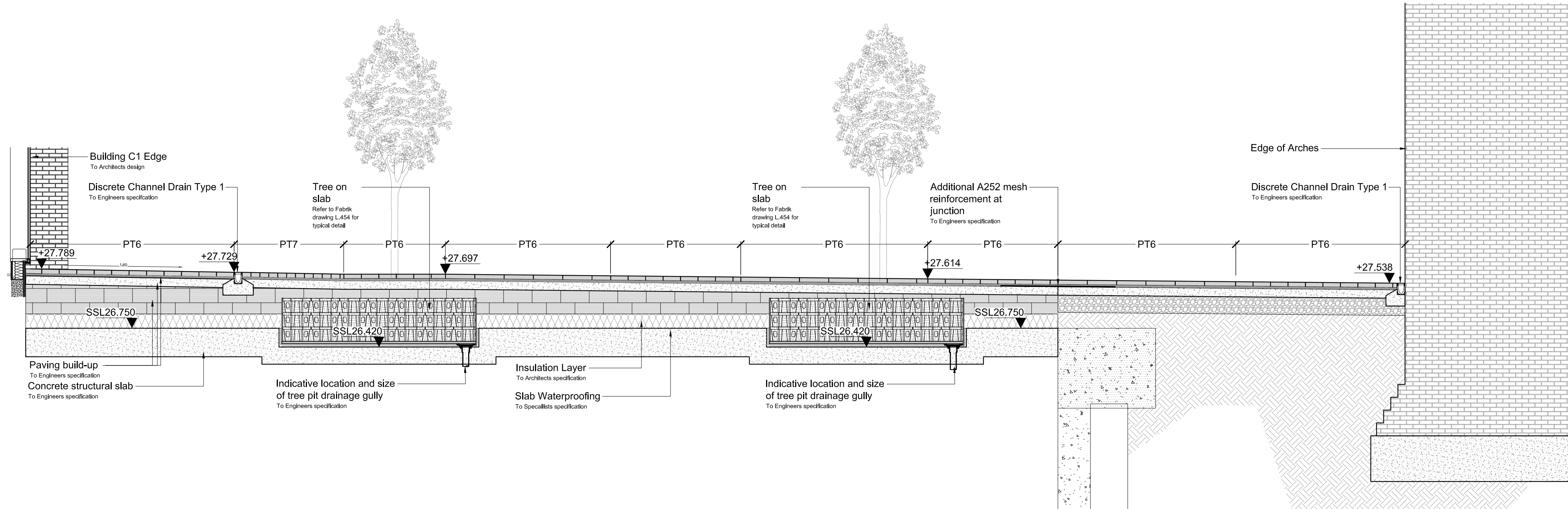
1 Building C1 - Section through local space SCALE 1:50@A1
