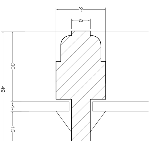
EXISTING WINDOW Detail 02 - Glazing Bar SCALE 1/1@A3
