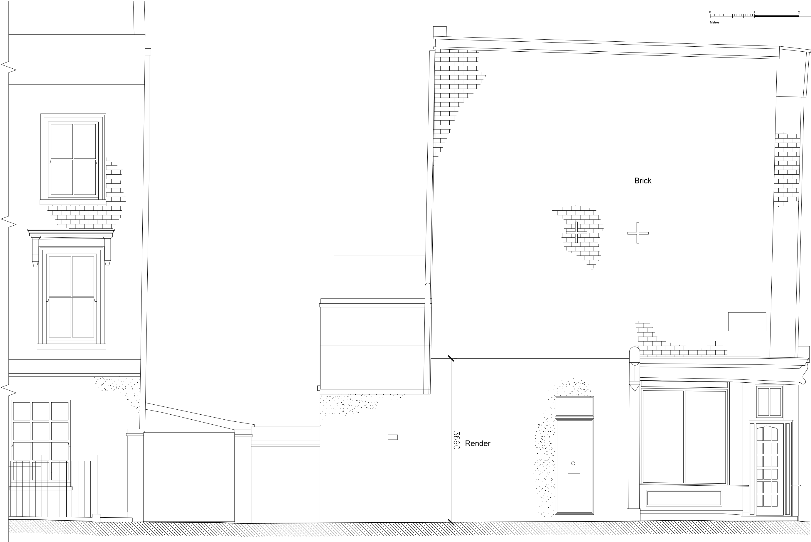
Side Elevation (Scale 1:50 @A3)
