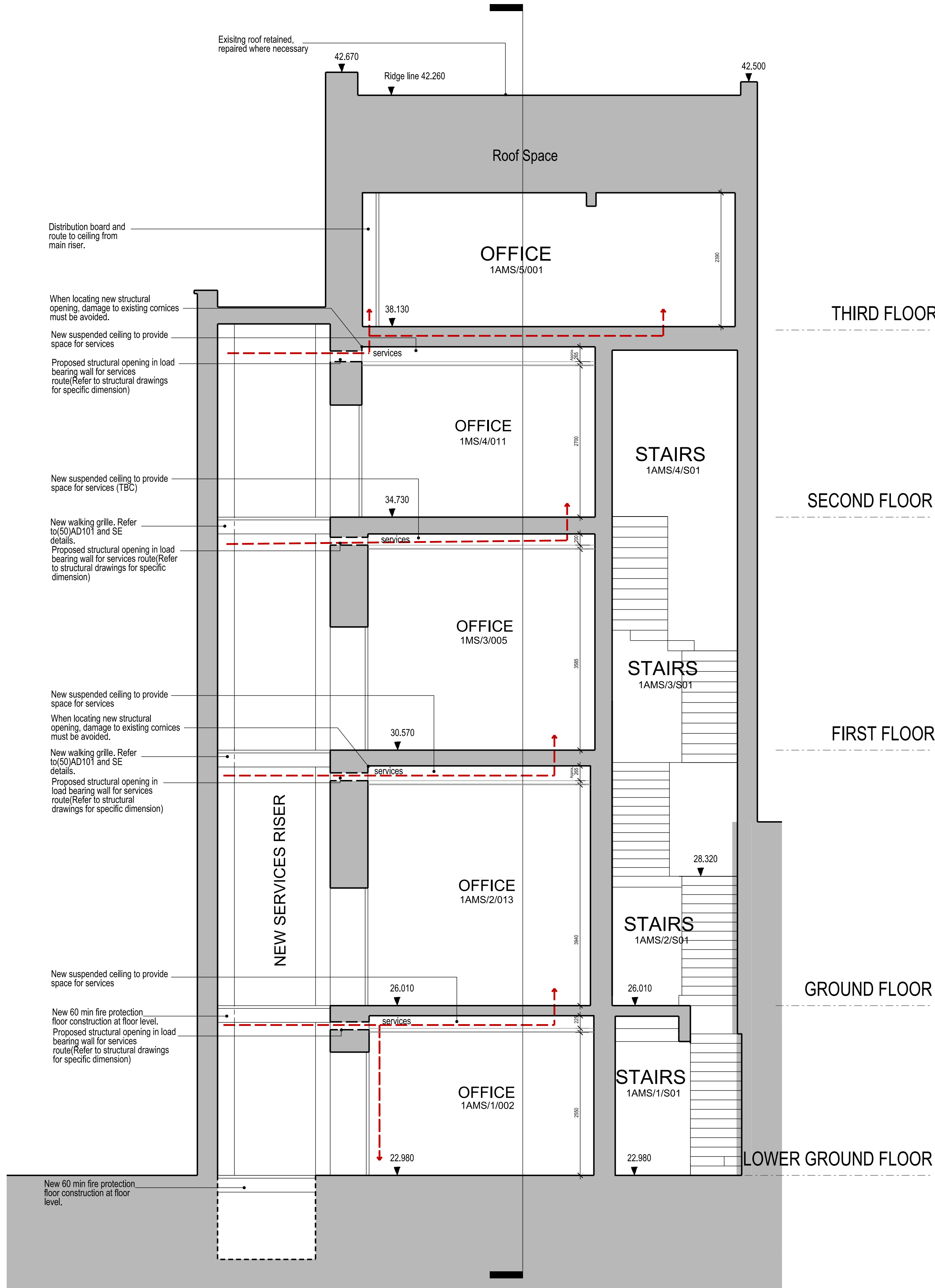
SECTION AA
