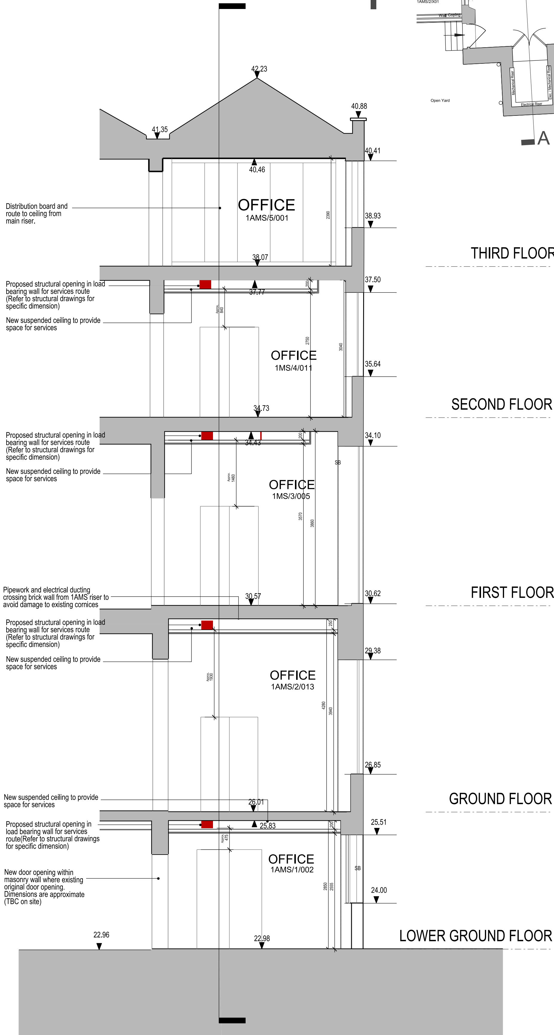
SECTION BB
