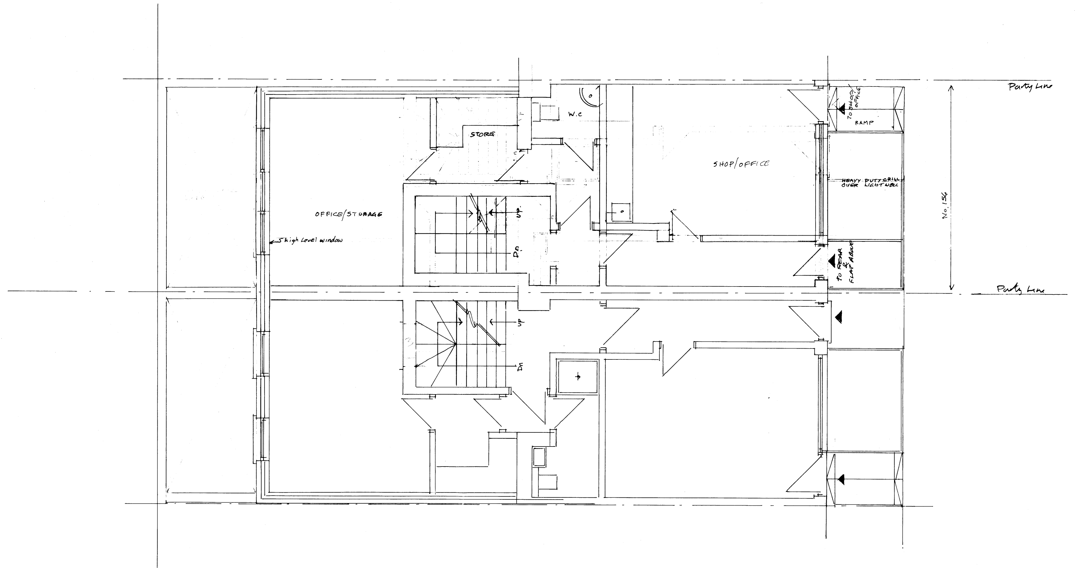
PROPOSED GROUND FLOOR PLAN 1:50 @ A2
