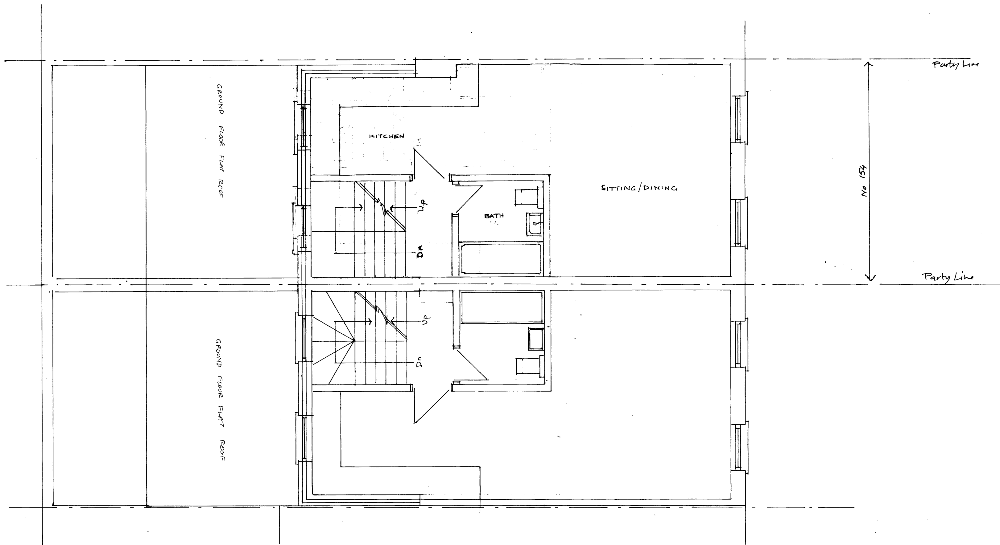
PROPOSED FIRST FLOOR PLAN 1:50 @ A2
