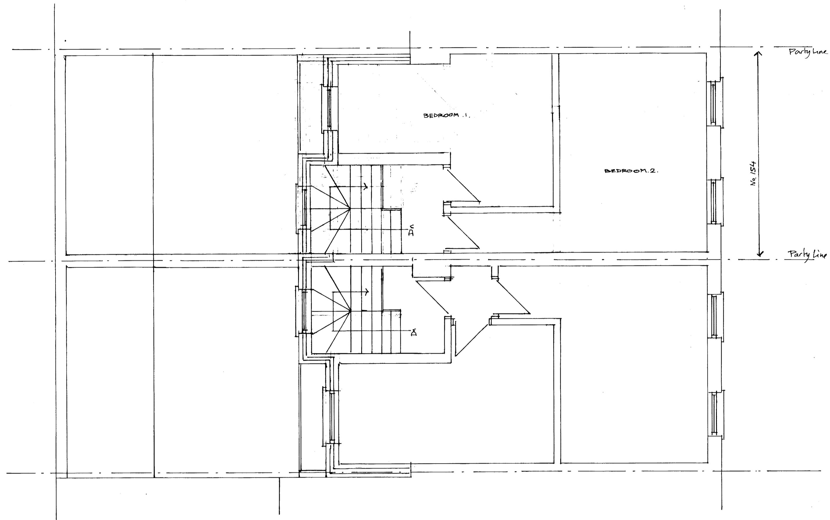
PROPOSED SECOND FLOOR PLAN 1:50 @ A2
