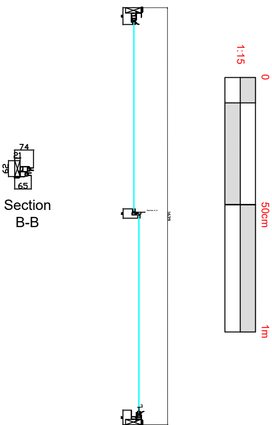
Secondary glazing Section A-A
