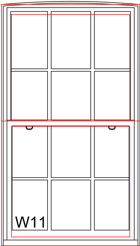
Window from inside with Secondary glazing
