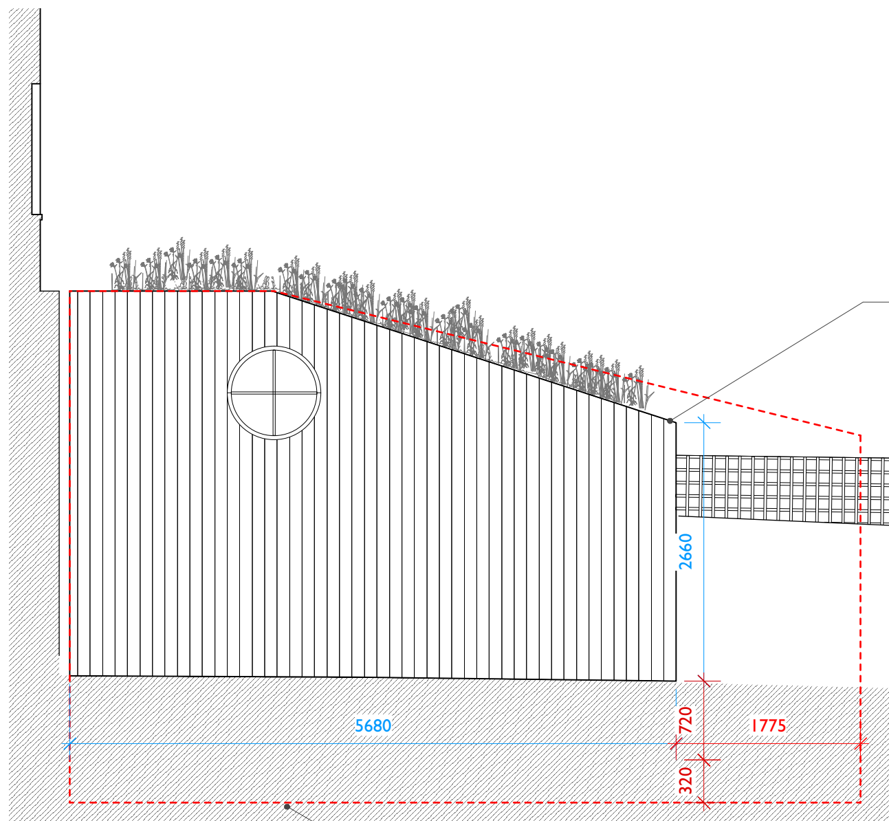
1 Garden Room Elevation E 05/21/1 1:50
