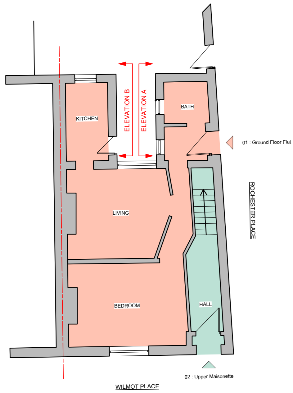
01 Existing Ground Floor Plan
