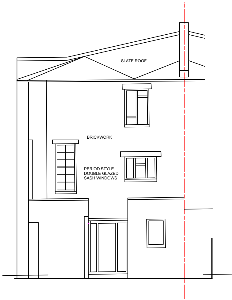
01 Existing Rear Elevation
