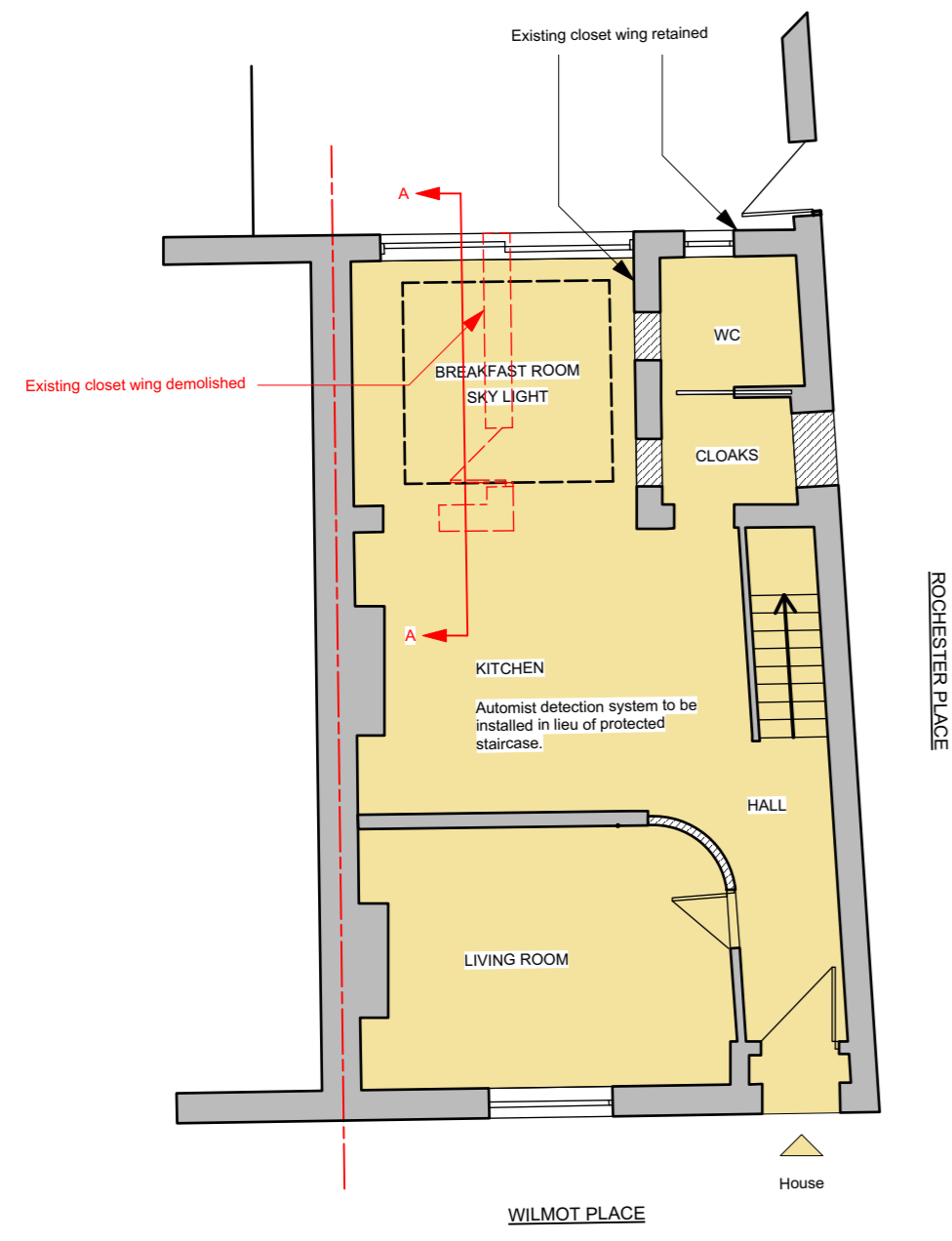
01 Proposed Ground Floor Plan
