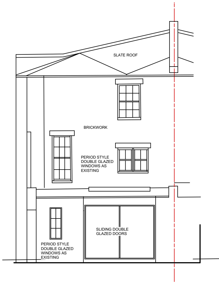
01 Proposed Rear Elevation
