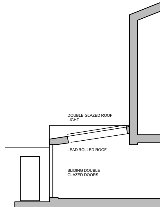
02 Proposed Section
