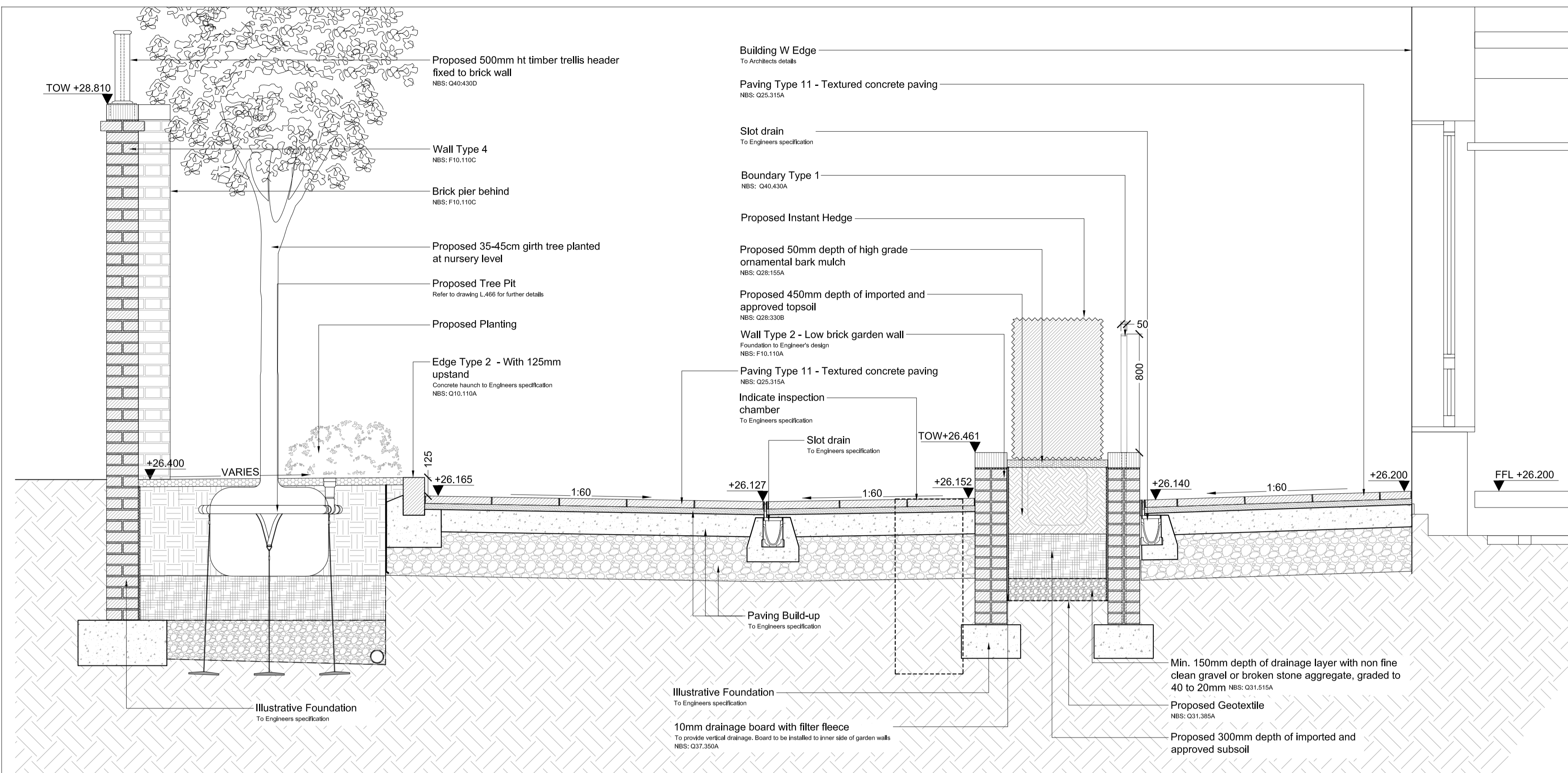
1 Building WX - Typical section through Rear Private Patios SCALE 1:20@A1
