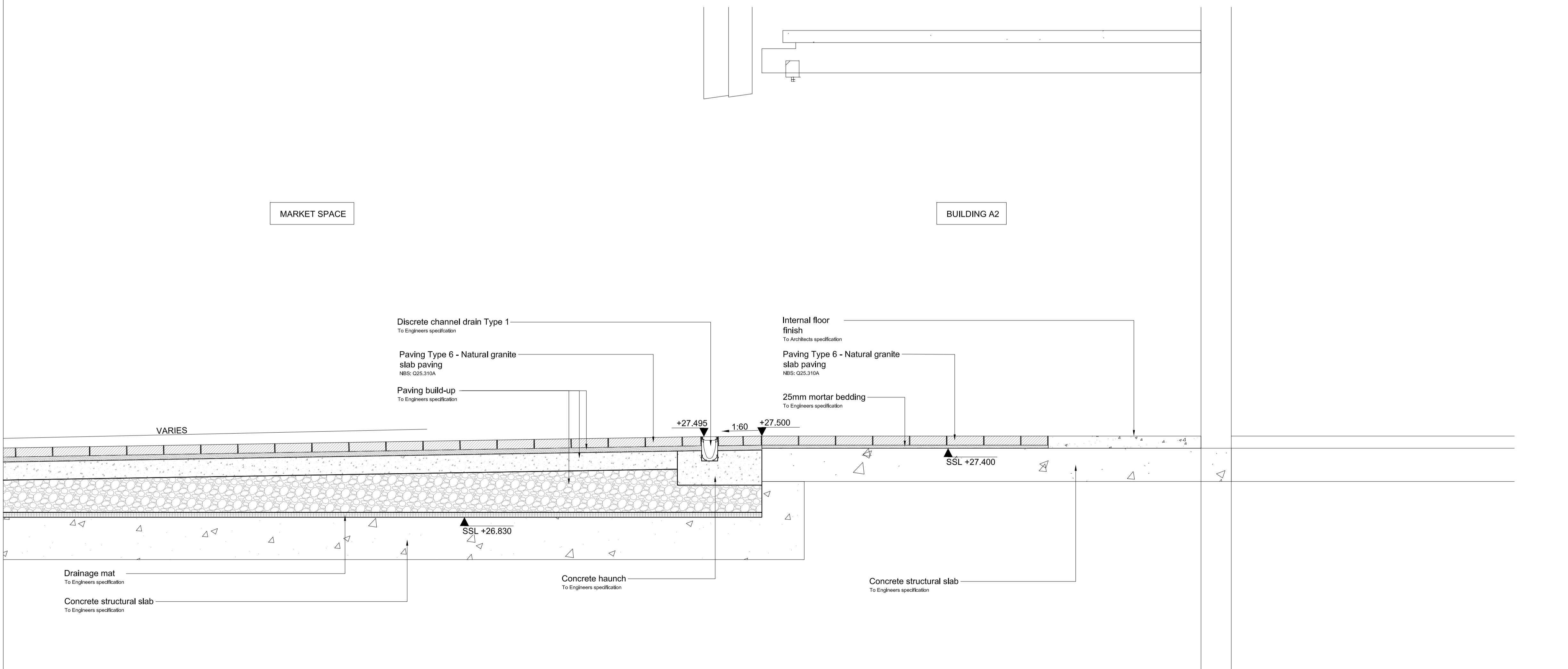
6 Market space - Entrance to Building A2 SCALE 1:20@A1
