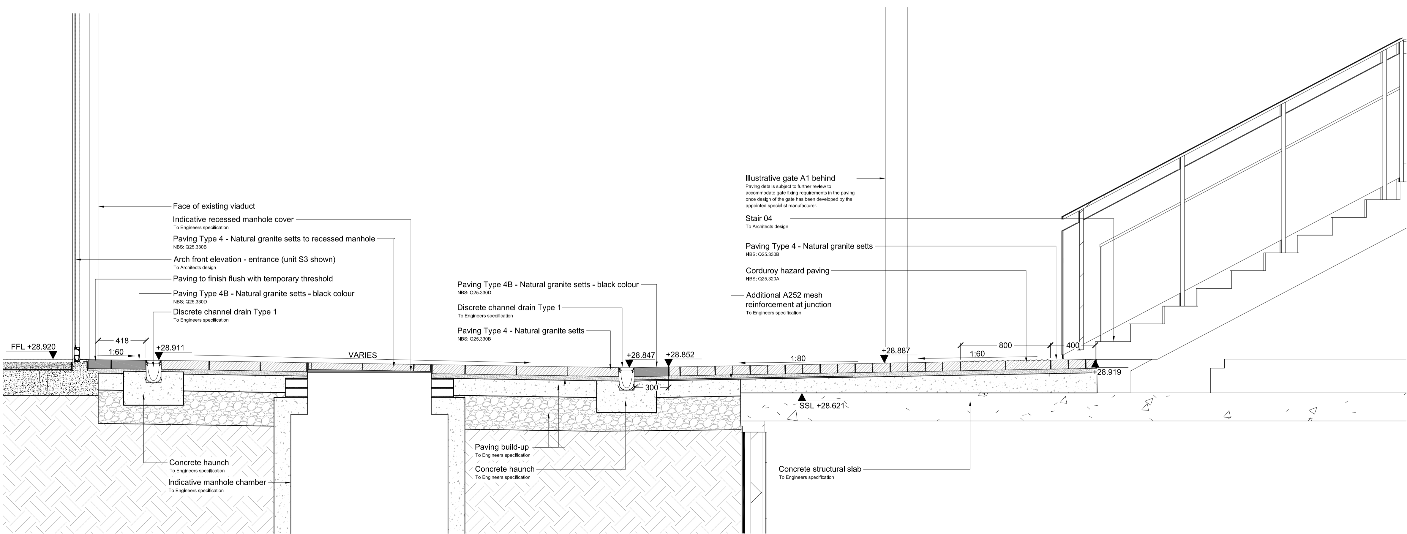
2 Section through Building A1 Stair 04 SCALE 1:20@A1
