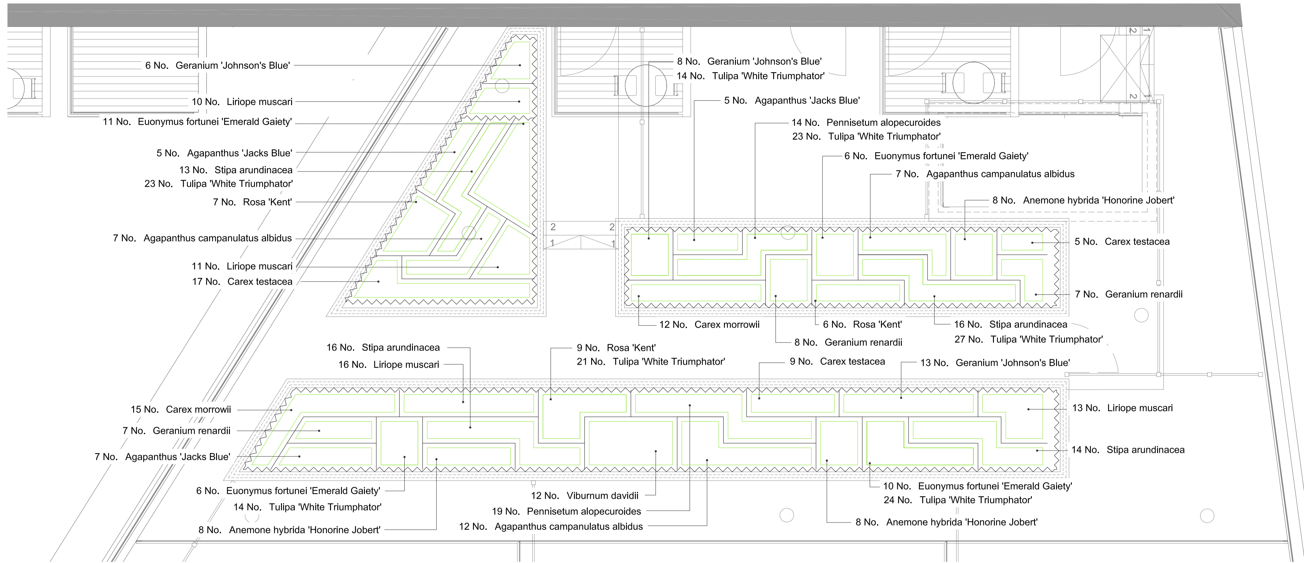
1 Building C1/C2: Level 2 Roof Terrace (C1) SCALE 1:50@A1
